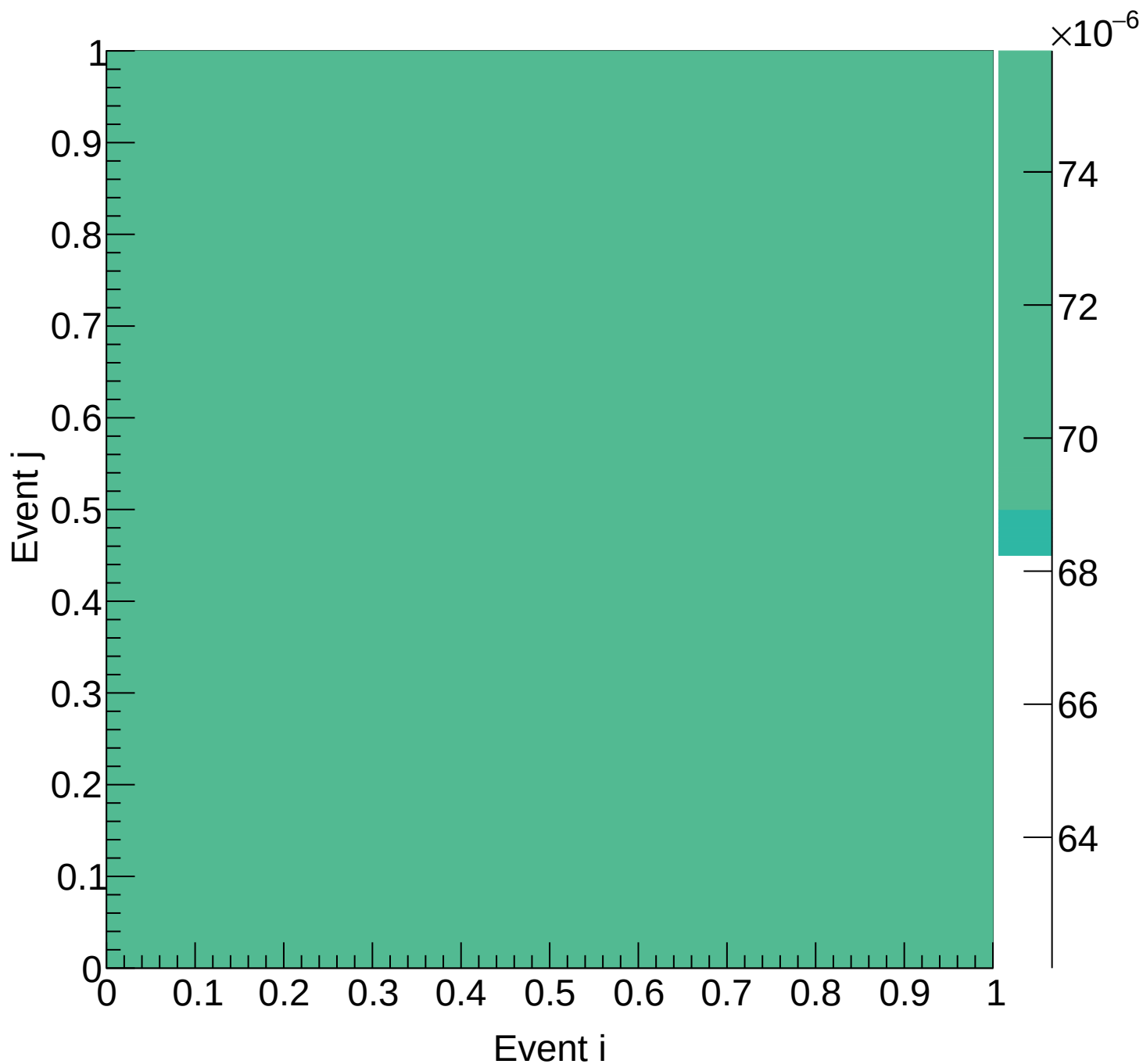
Flask (total) Covariance | M: [3.9, 4.2) xF: [0.80, 0.85)
