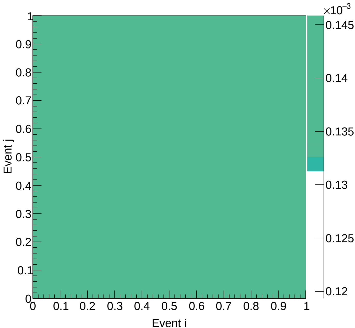
Flask (total) Covariance | M: [3.9, 4.2) xF: [0.85, 0.90)
