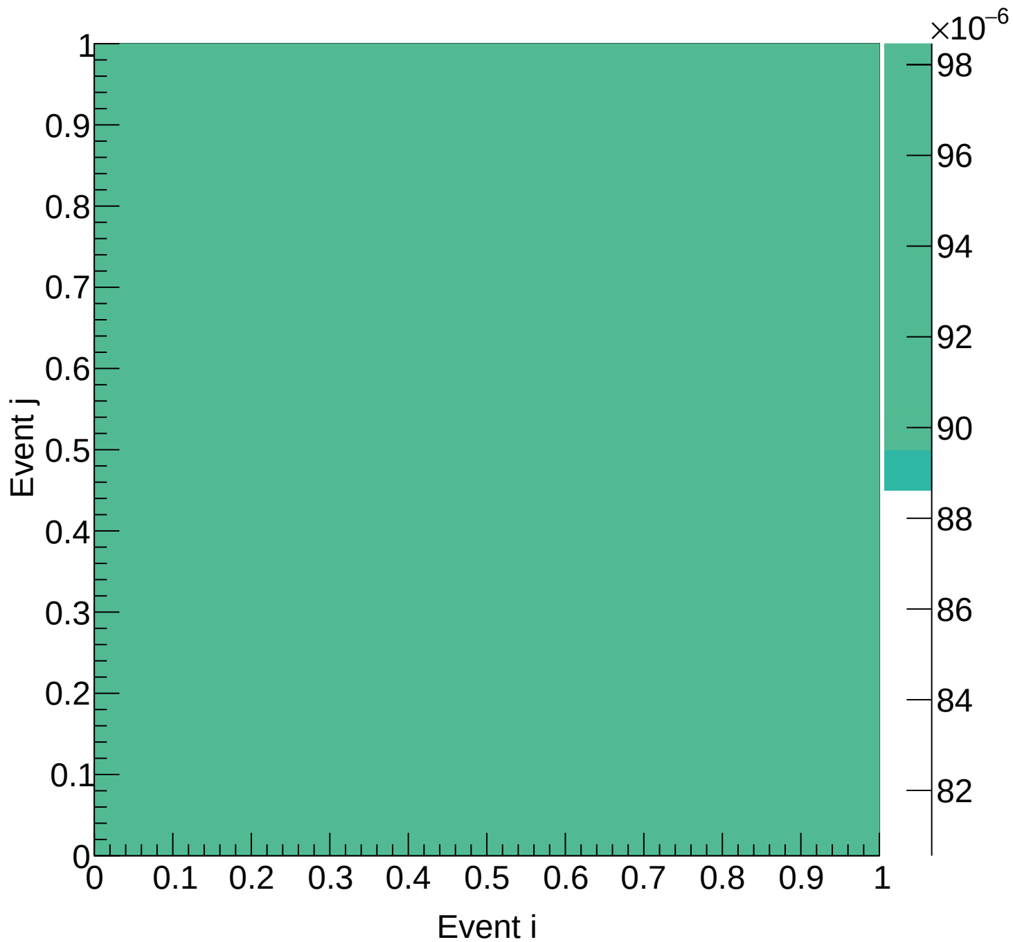
Flask (total) Covariance | M: [4.2, 4.5) xF: [0.85, 0.90)
