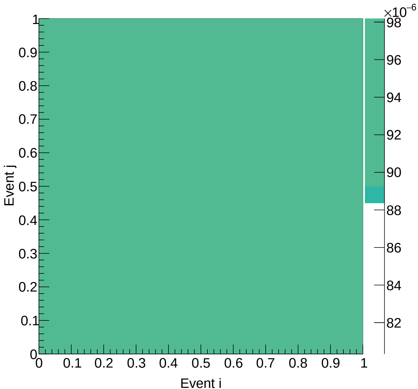
Flask (total) Covariance | M: [4.5, 4.8) xF: [0.85, 0.90)
