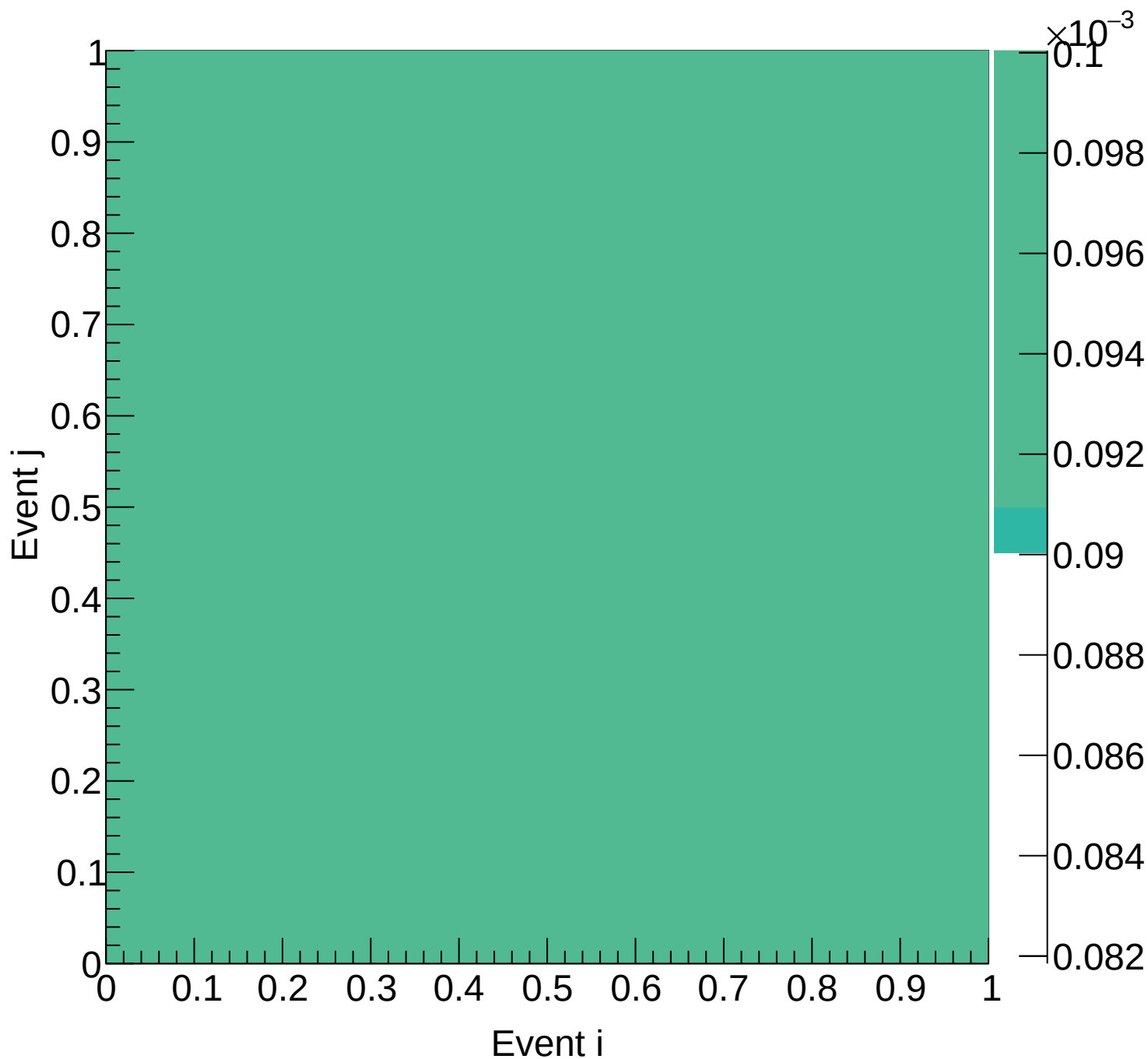
Flask (total) Covariance | M: [3.9, 4.2) xF: [0.90, 0.95)
