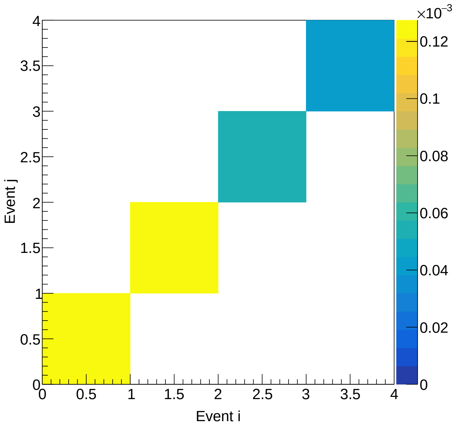
Flask (total) Covariance | M: [4.5, 4.8) xF: [0.05, 0.10)
