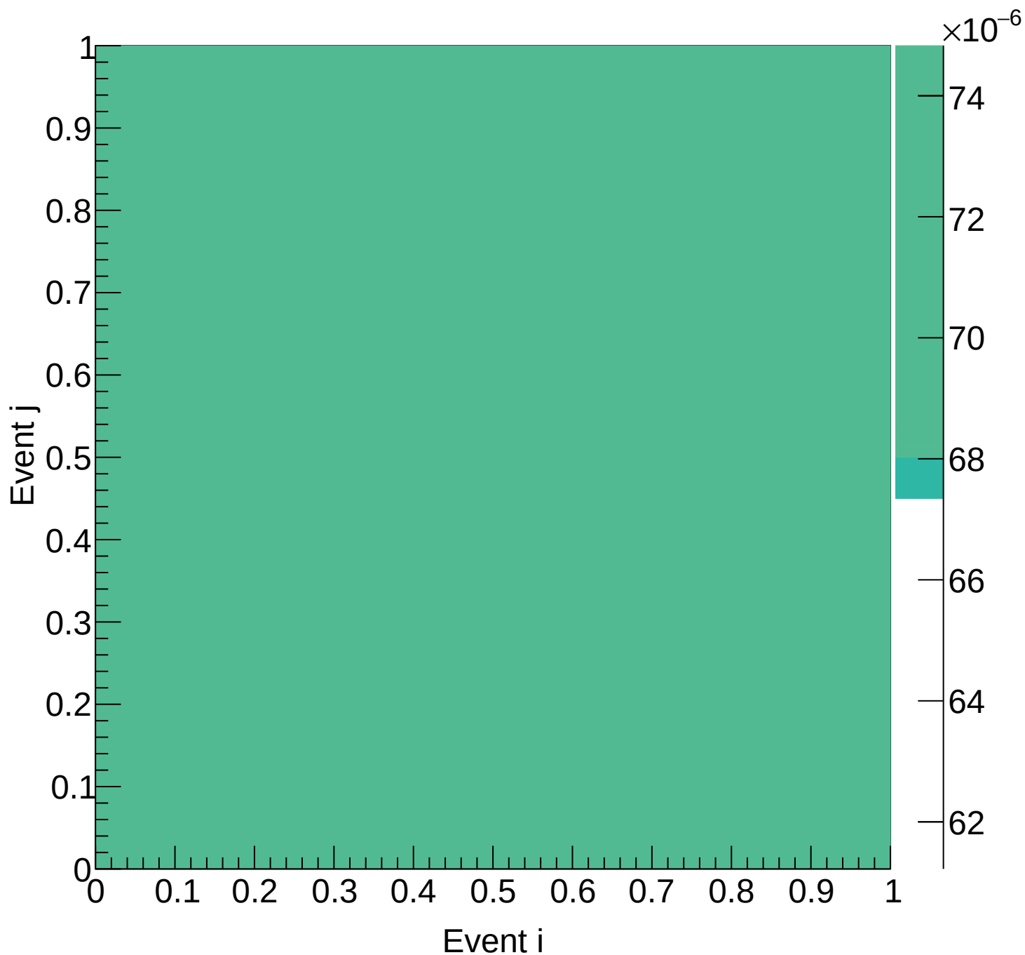
Flask (total) Covariance | M: [6.3, 6.6) xF: [0.05, 0.10)
