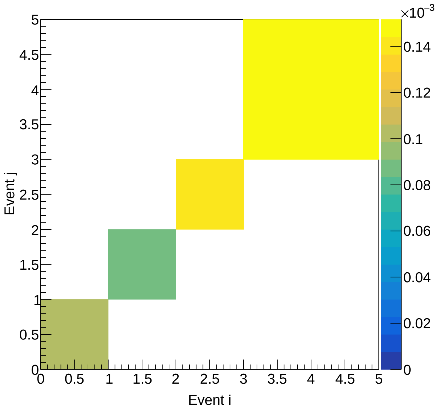
Flask (total) Covariance | M: [4.5, 4.8) xF: [0.10, 0.15)
