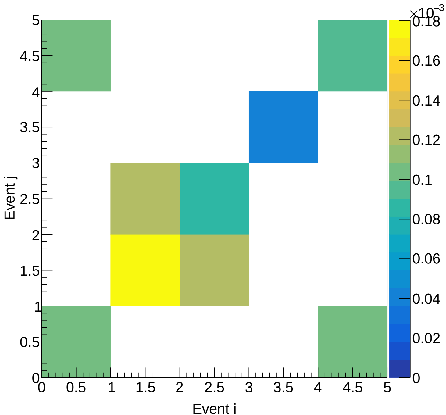
Flask (total) Covariance | M: [5.1, 5.4) xF: [0.10, 0.15)
