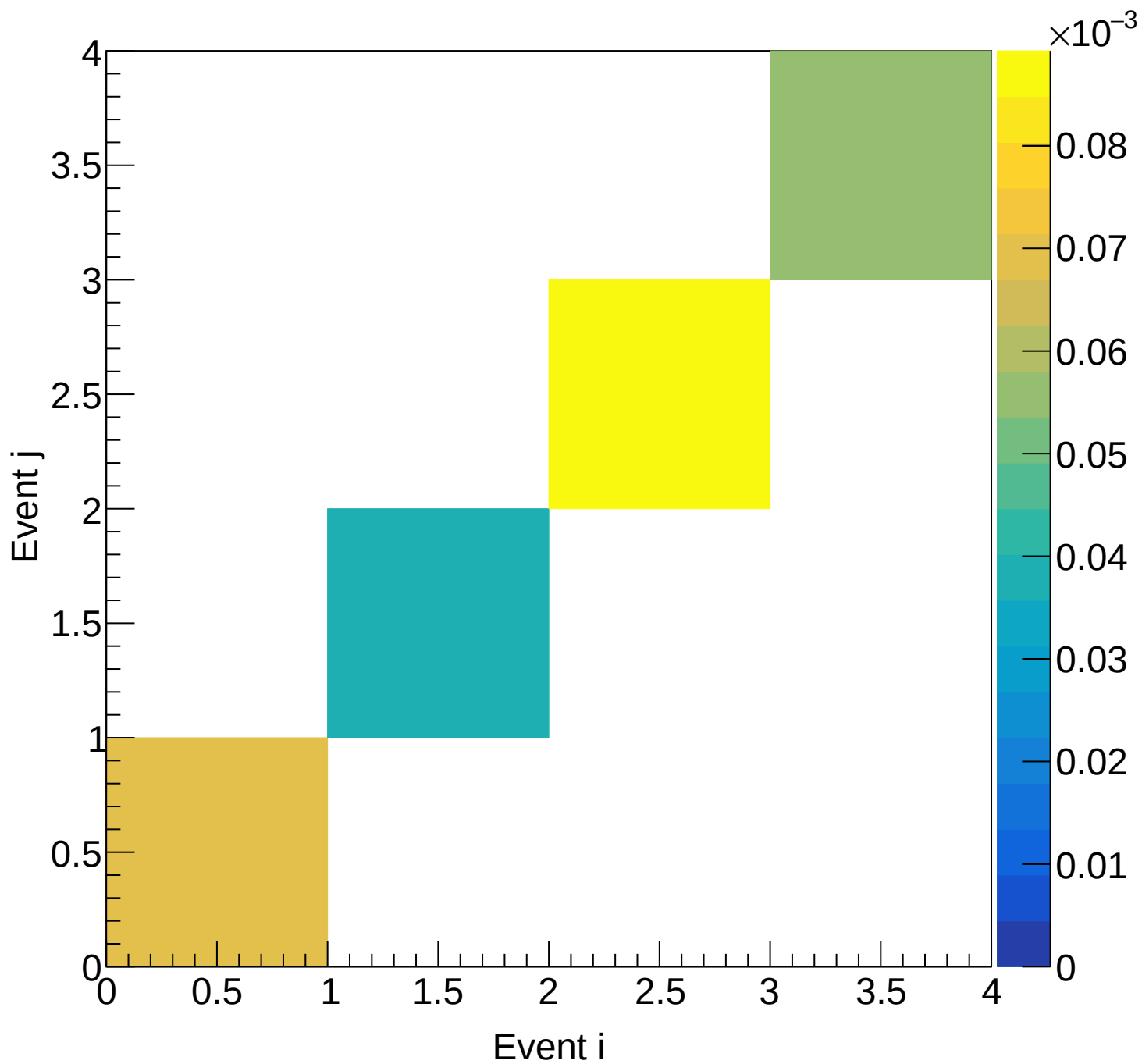
Flask (total) Covariance | M: [5.7, 6.0) xF: [0.10, 0.15)
