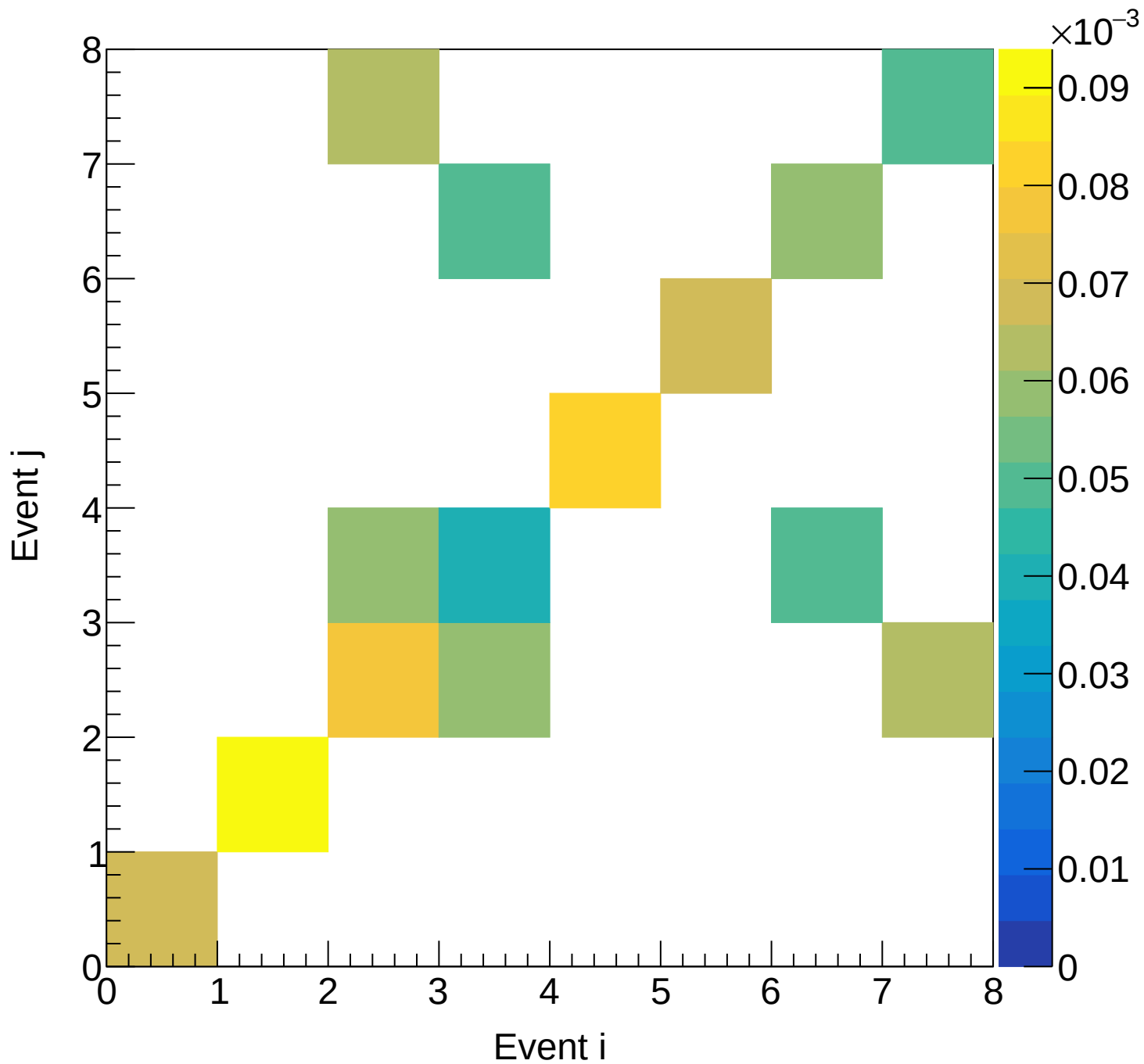
Flask (total) Covariance | M: [4.5, 4.8) xF: [0.15, 0.20)
