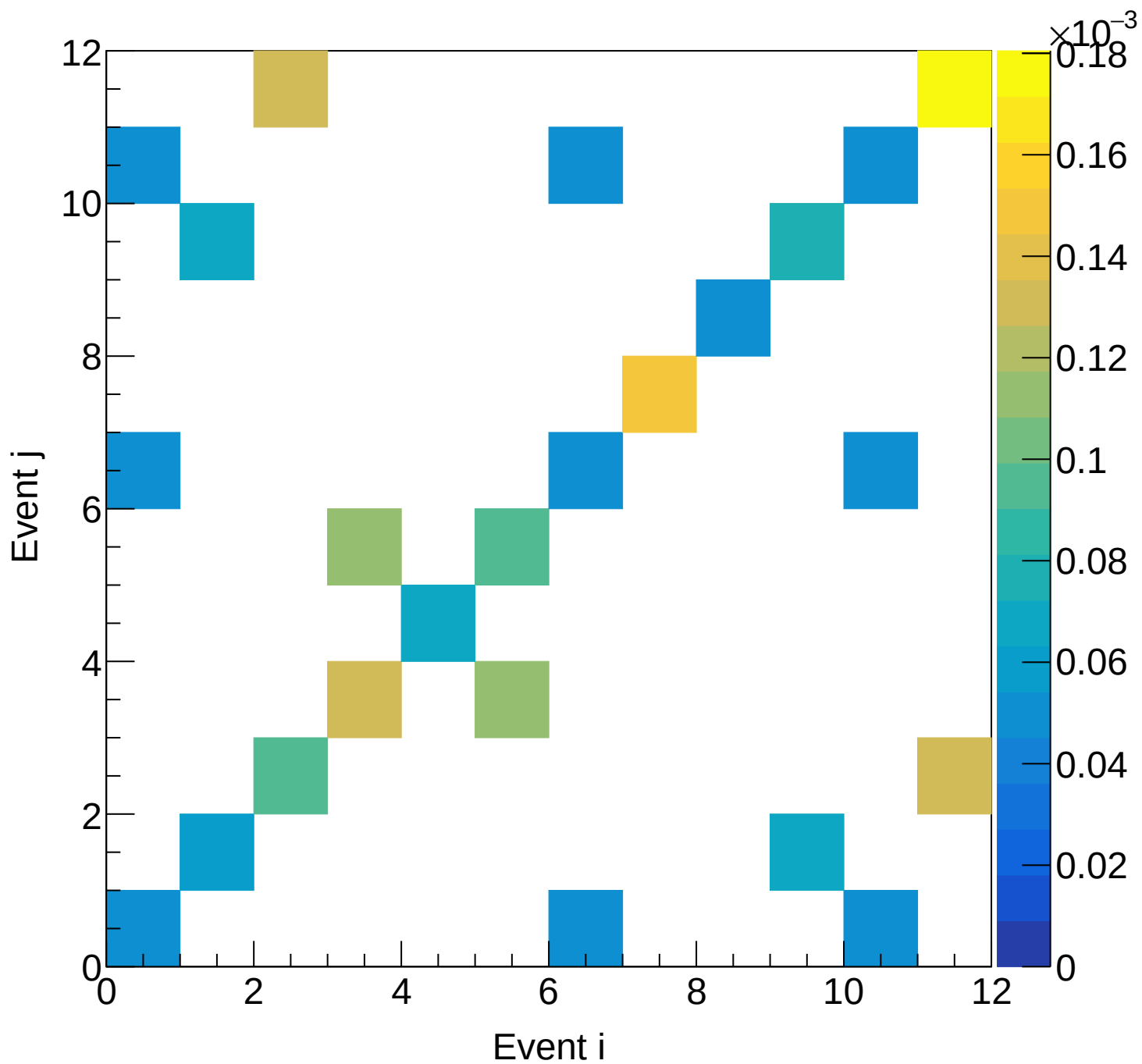
Flask (total) Covariance | M: [4.2, 4.5) xF: [0.20, 0.25)
