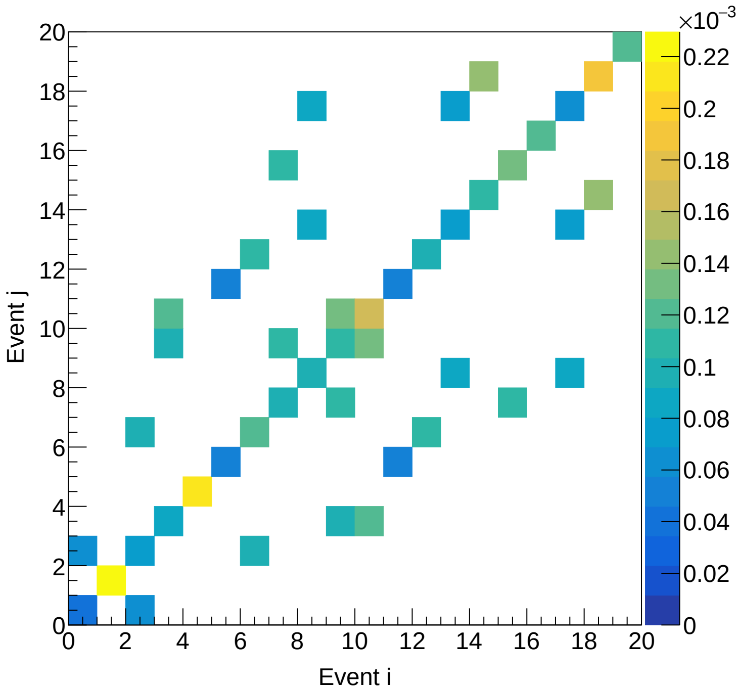
Flask (total) Covariance | M: [4.5, 4.8) xF: [0.20, 0.25)
