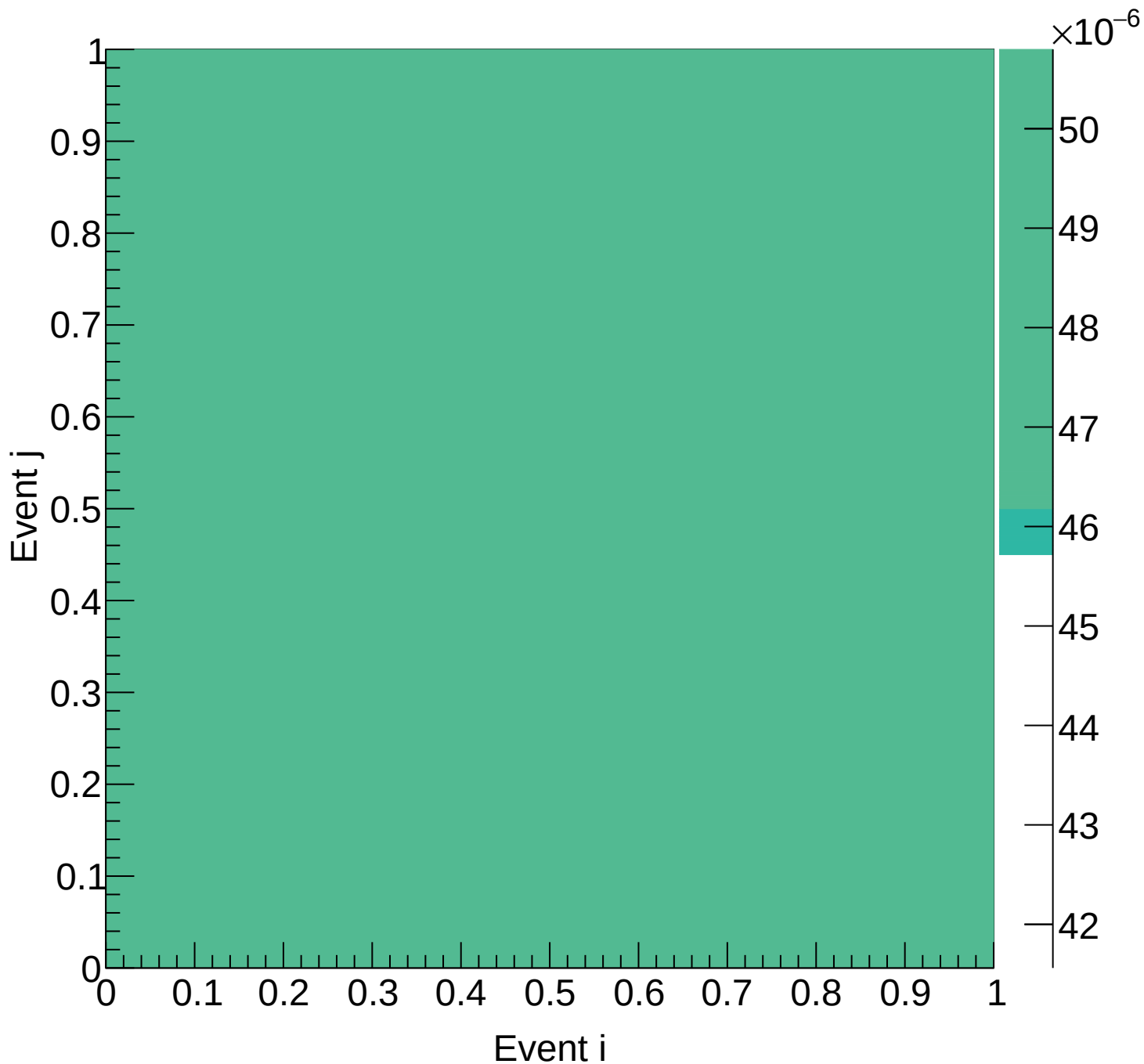
Flask (total) Covariance | M: [6.3, 6.6) xF: [0.20, 0.25)
