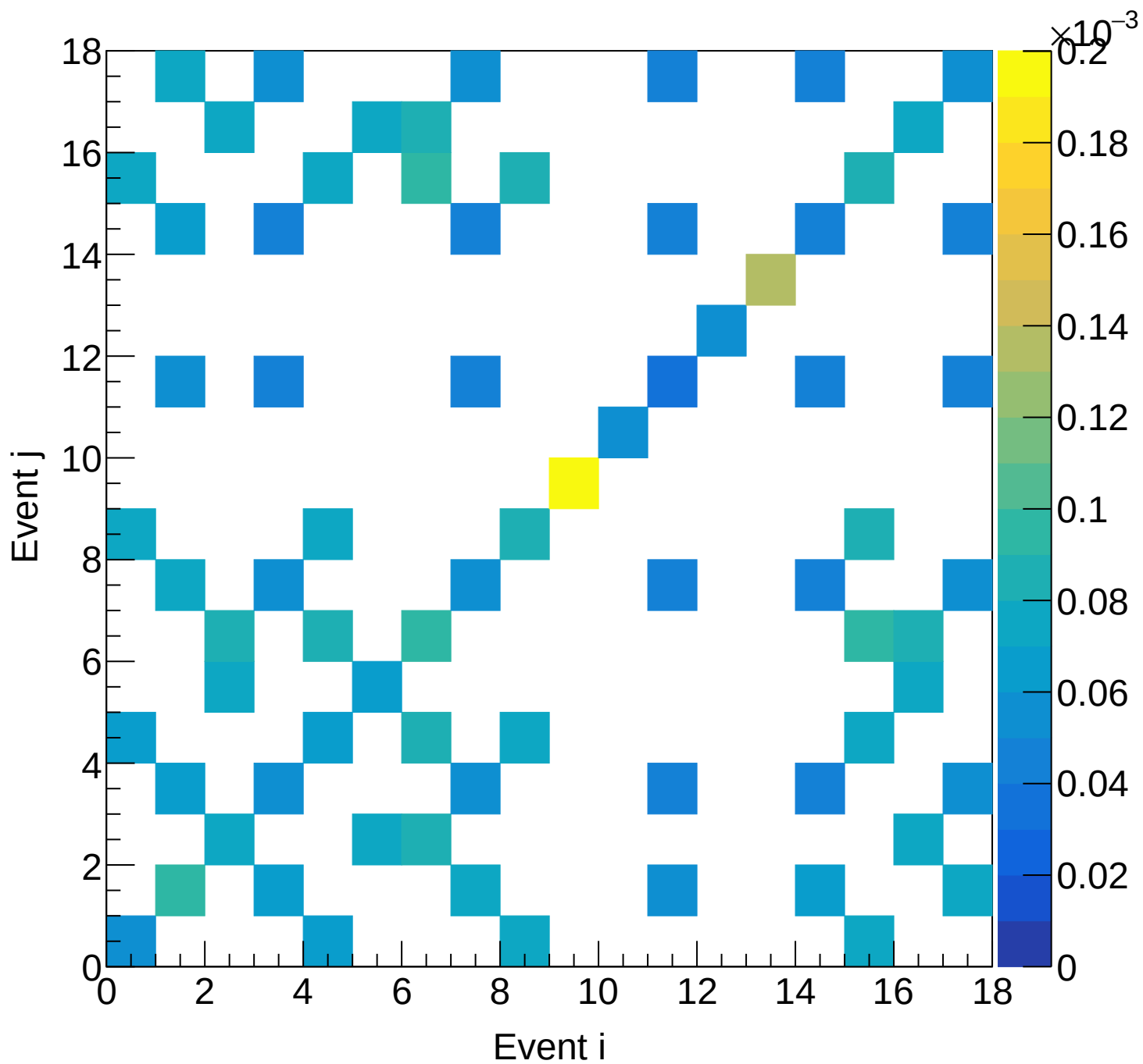
Flask (total) Covariance | M: [4.5, 4.8) xF: [0.25, 0.30)
