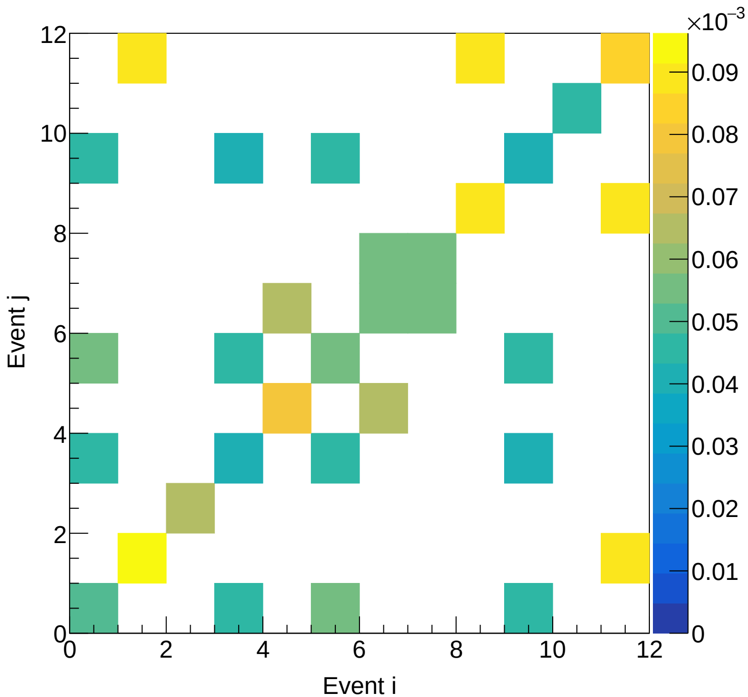
Flask (total) Covariance | M: [4.8, 5.1) xF: [0.25, 0.30)
