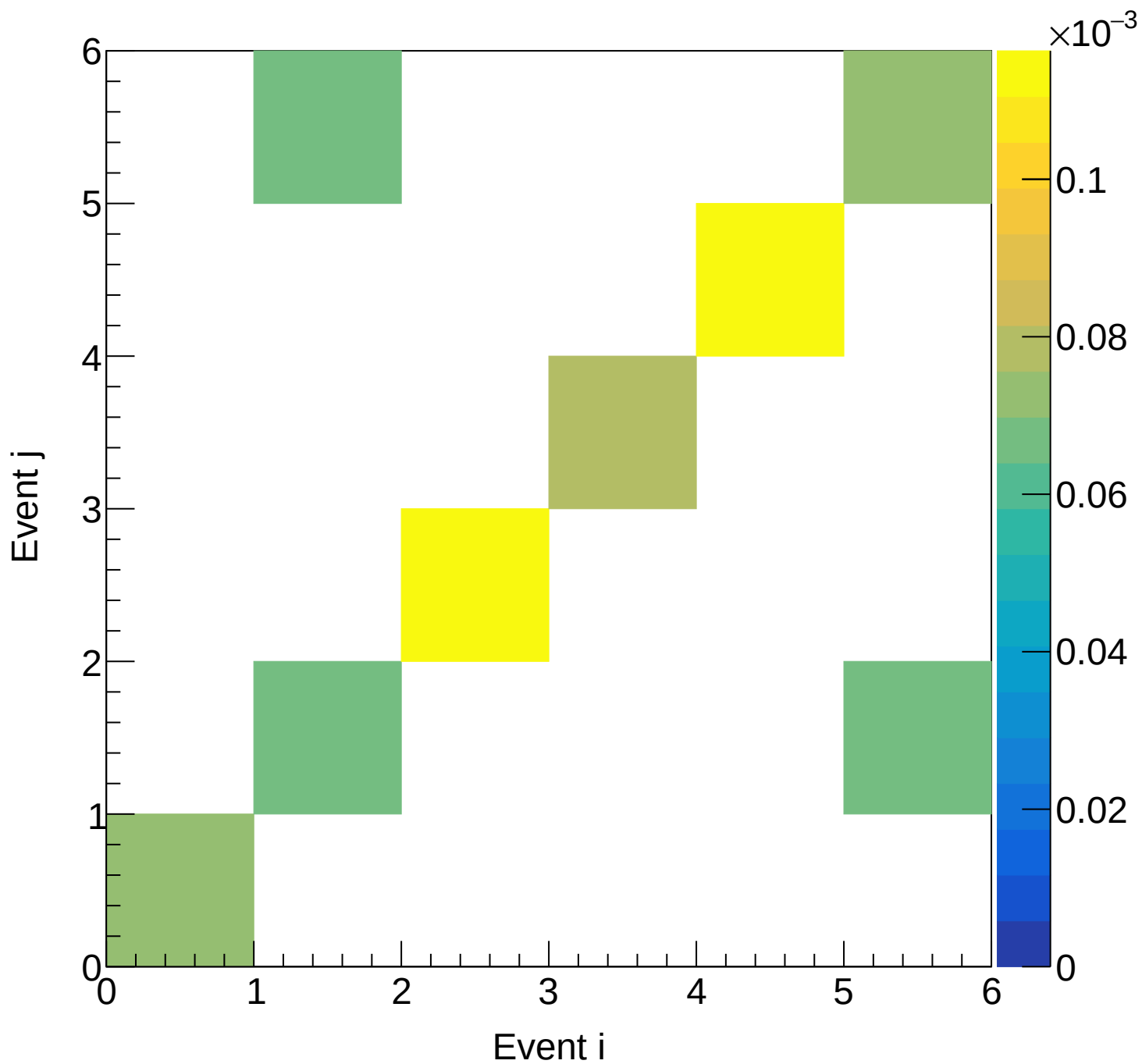
Flask (total) Covariance | M: [5.1, 5.4) xF: [0.25, 0.30)
