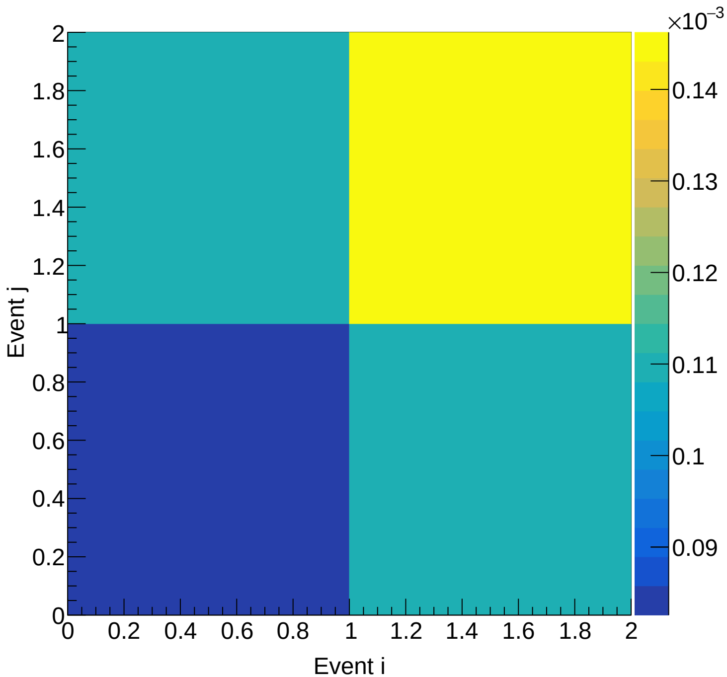
Flask (total) Covariance | M: [6.3, 6.6) xF: [0.25, 0.30)
