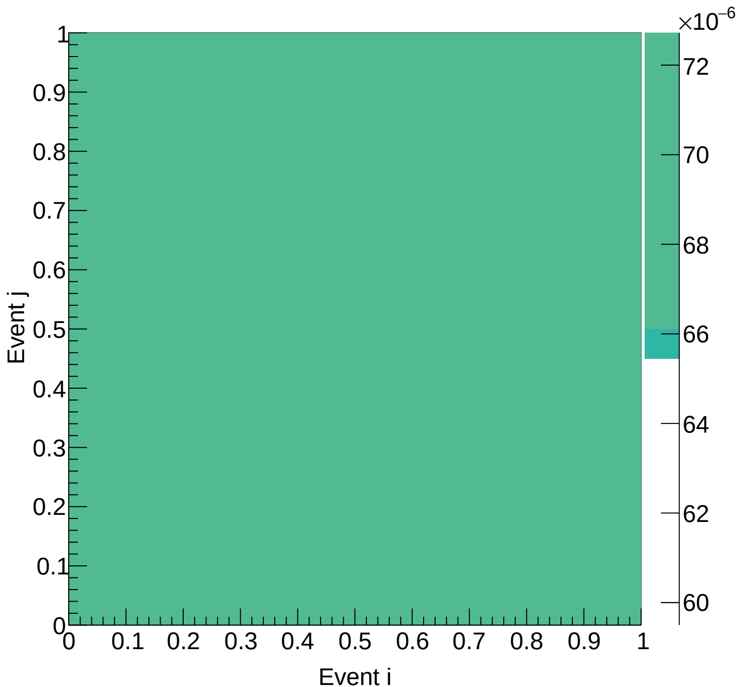
Flask (total) Covariance | M: [6.6, 6.9) xF: [0.25, 0.30)
