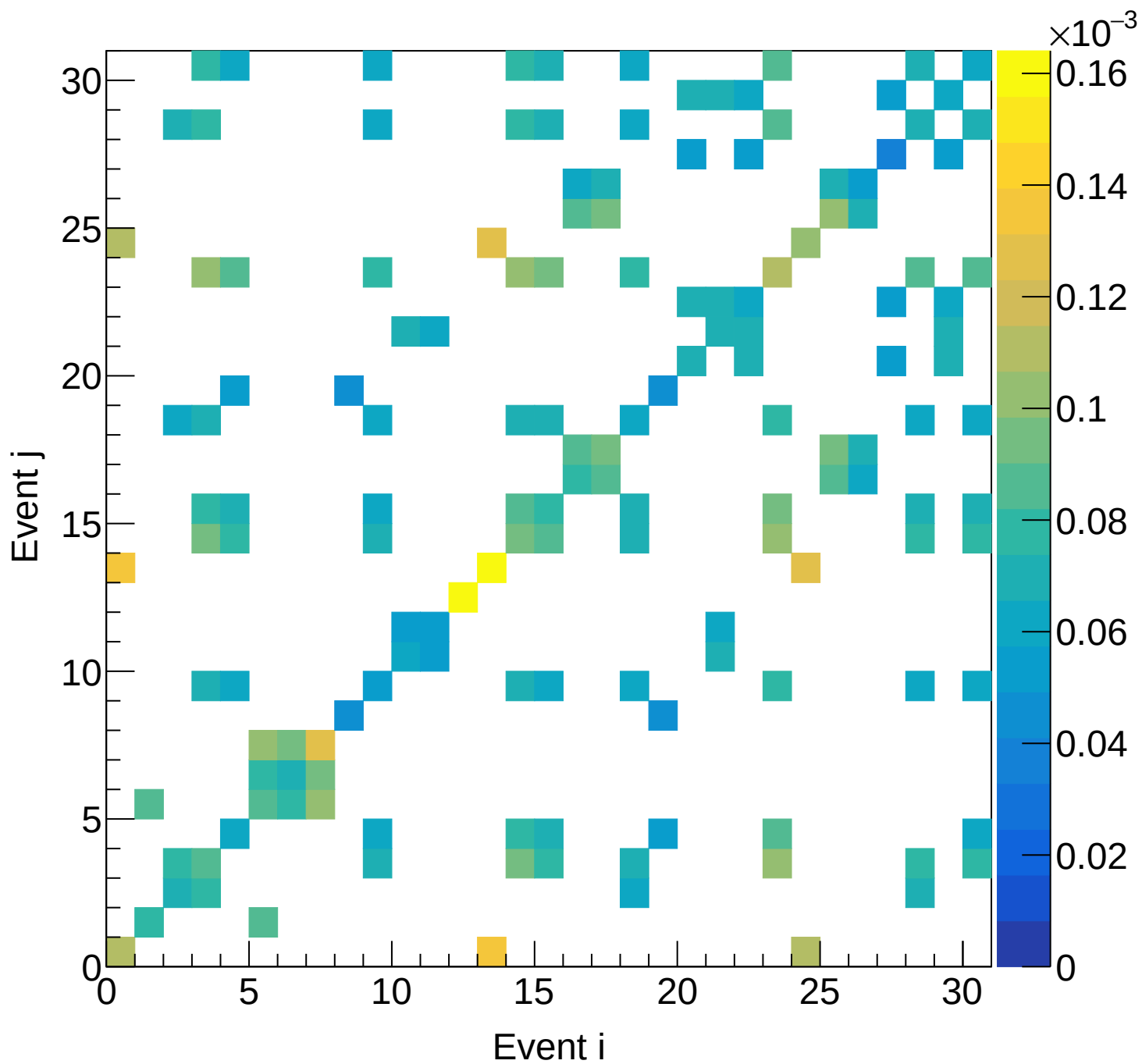
Flask (total) Covariance | M: [3.9, 4.2) xF: [0.30, 0.35)
