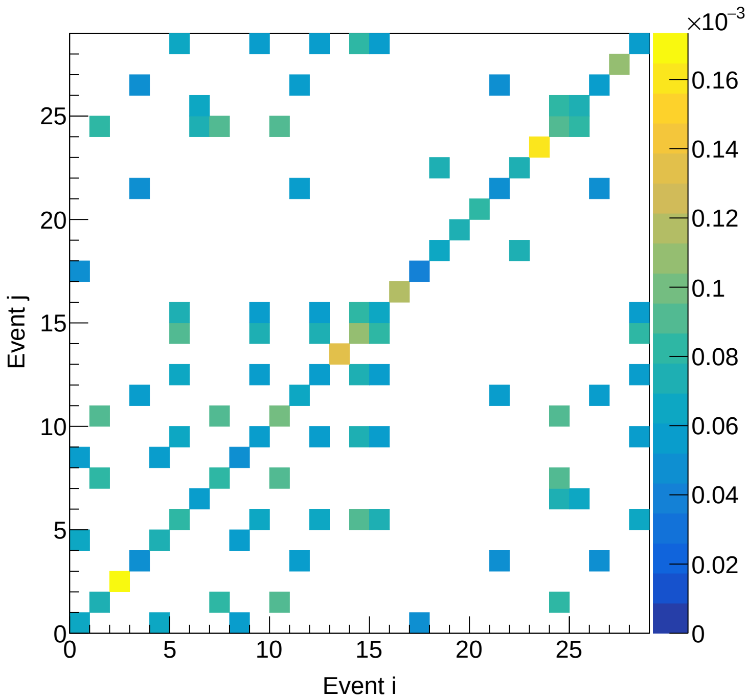
Flask (total) Covariance | M: [4.2, 4.5) xF: [0.30, 0.35)
