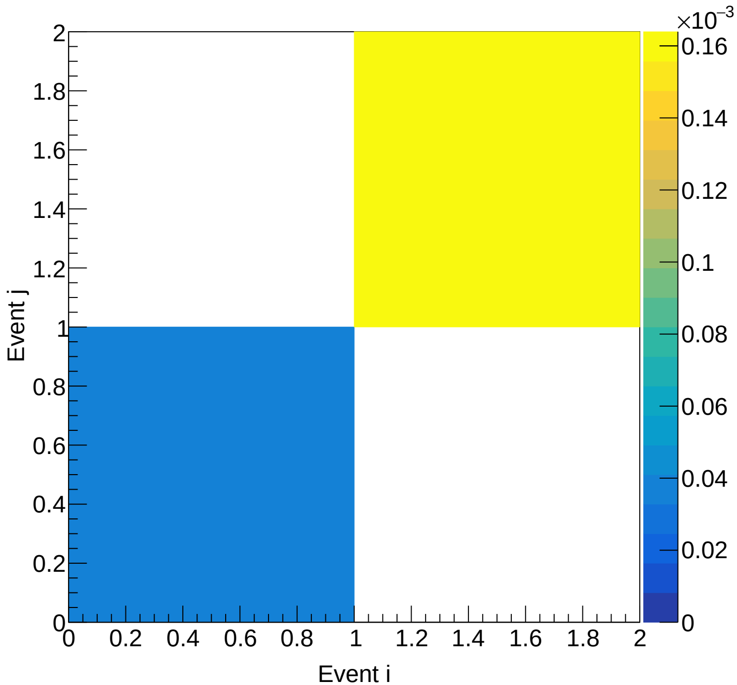
Flask (total) Covariance | M: [6.3, 6.6) xF: [0.30, 0.35)
