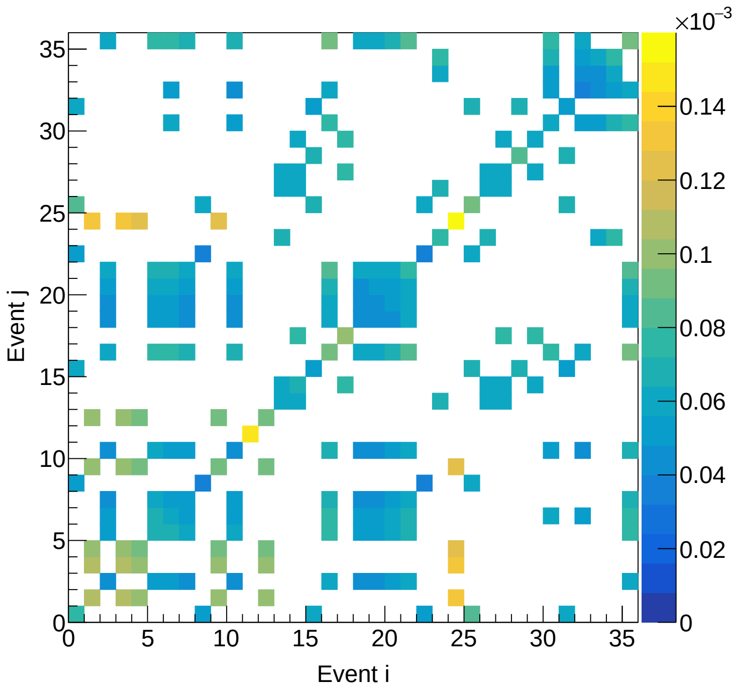
Flask (total) Covariance | M: [3.9, 4.2) xF: [0.35, 0.40)
