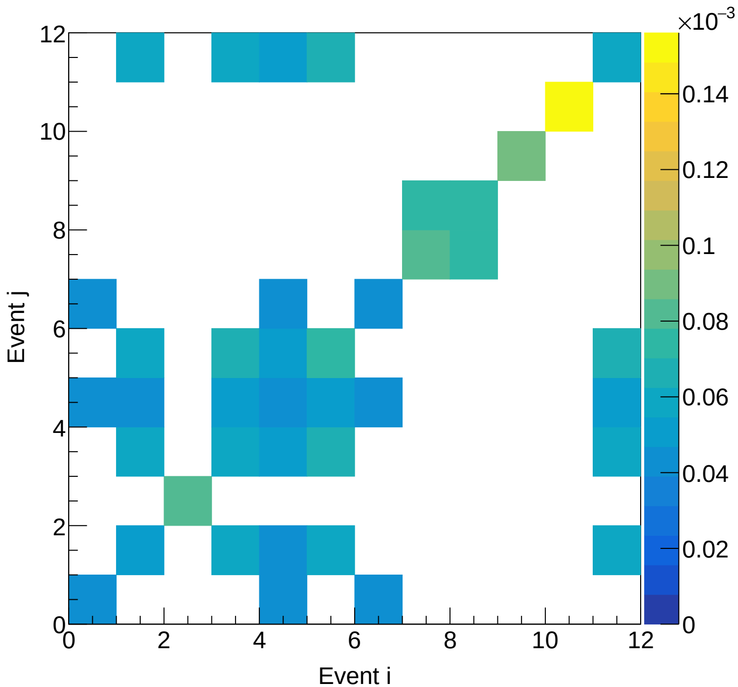
Flask (total) Covariance | M: [4.8, 5.1) xF: [0.35, 0.40)
