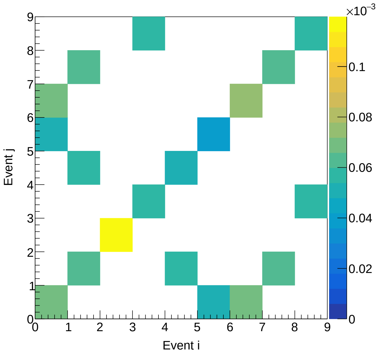
Flask (total) Covariance | M: [5.4, 5.7) xF: [0.35, 0.40)
