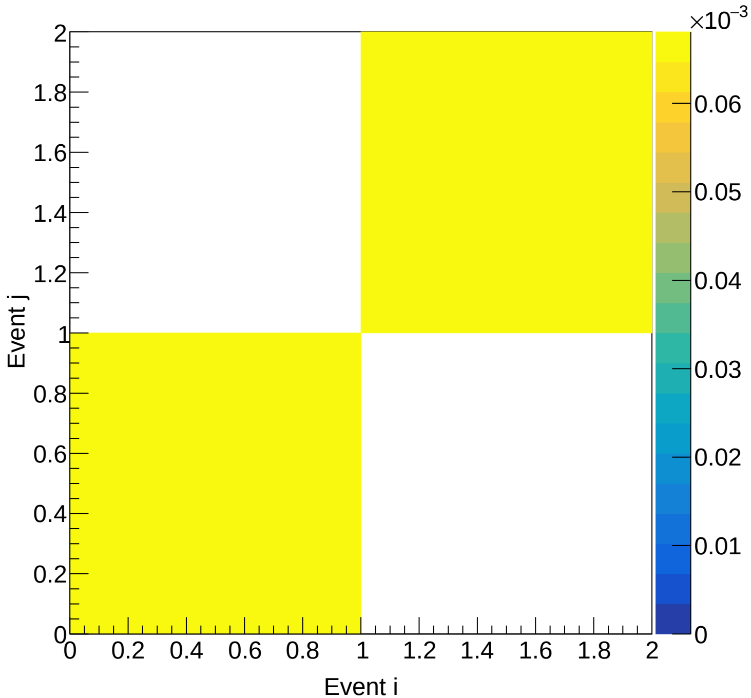
Flask (total) Covariance | M: [6.0, 6.3) xF: [0.35, 0.40)
