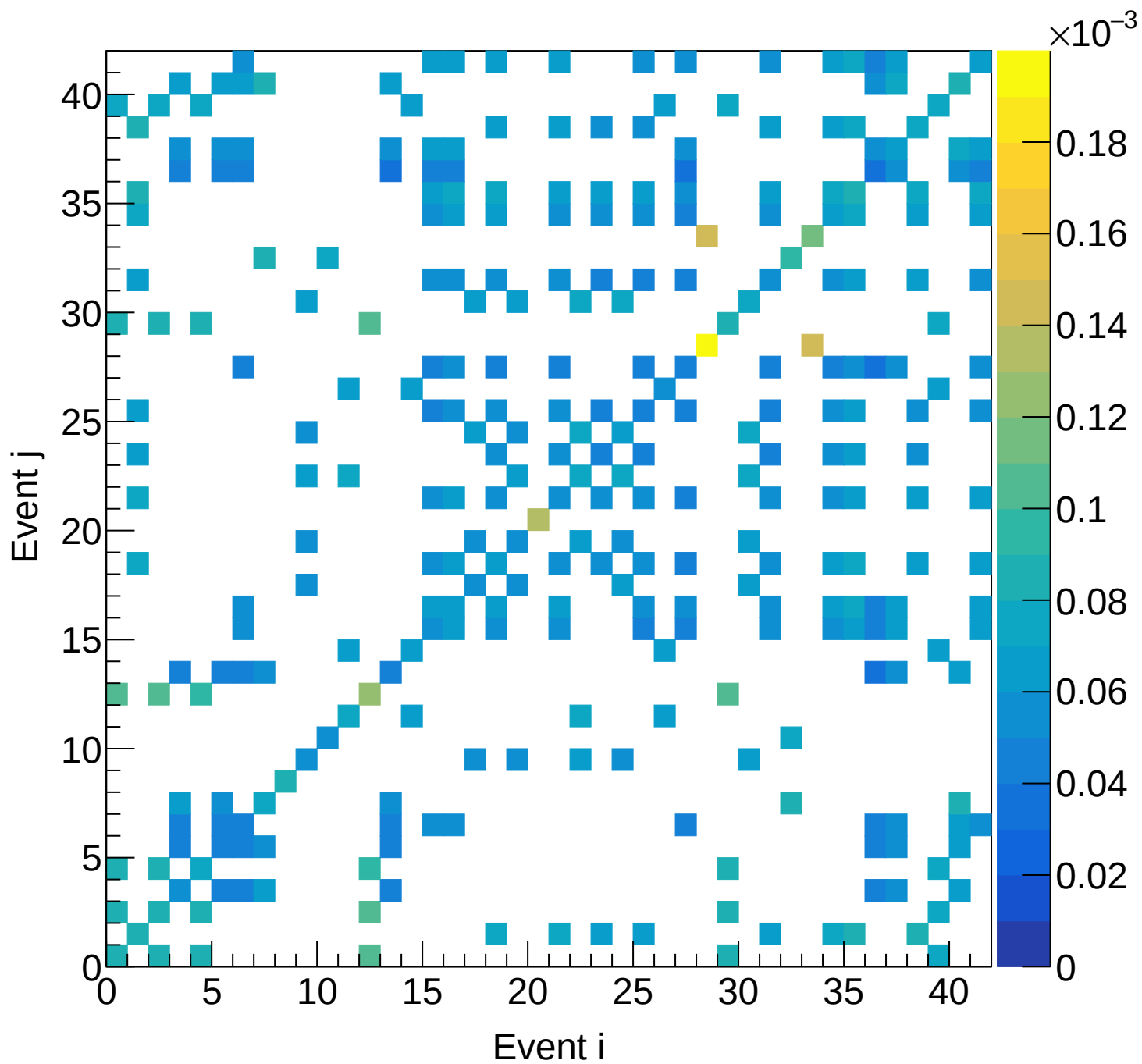
Flask (total) Covariance | M: [3.9, 4.2) xF: [0.40, 0.45)
