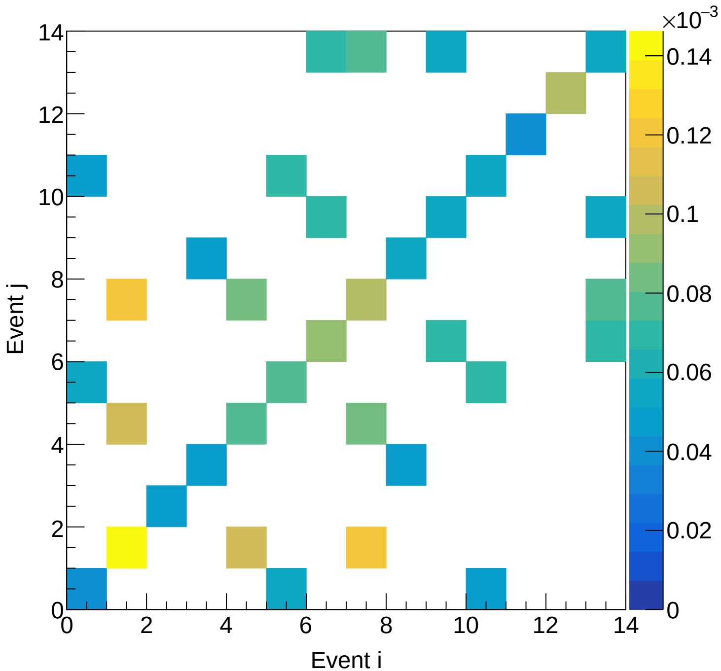
Flask (total) Covariance | M: [4.8, 5.1) xF: [0.40, 0.45)
