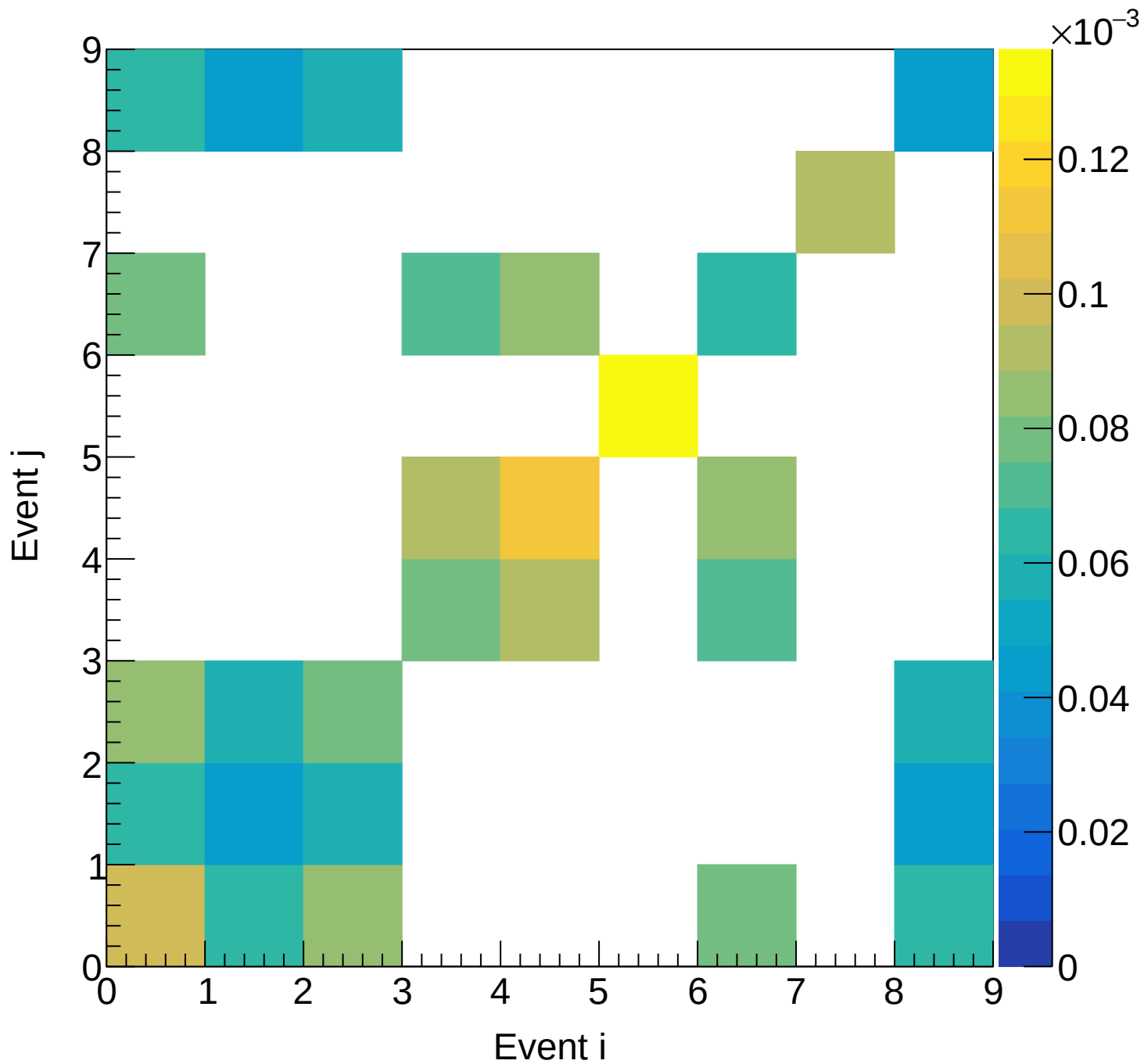
Flask (total) Covariance | M: [5.1, 5.4) xF: [0.40, 0.45)
