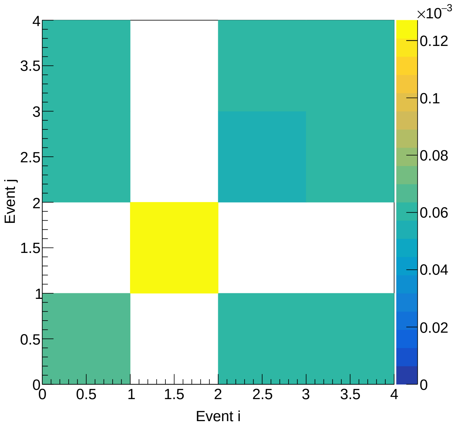
Flask (total) Covariance | M: [5.4, 5.7) xF: [0.40, 0.45)
