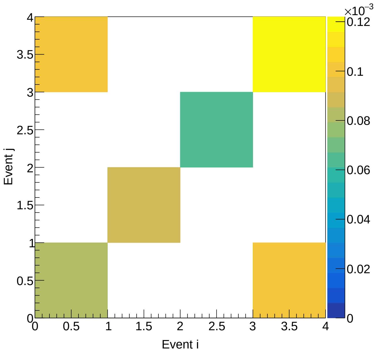
Flask (total) Covariance | M: [5.7, 6.0) xF: [0.40, 0.45)
