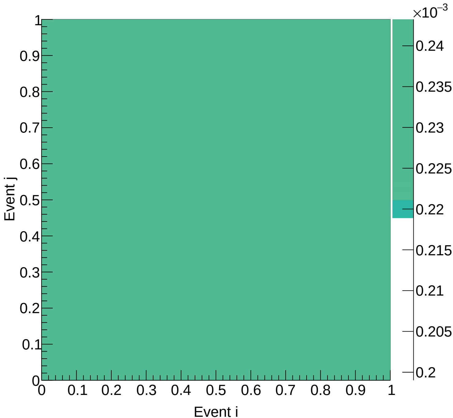
LD2 (mix) Covariance | M: [6.9, 7.5] xF: [-0.05, 0.00)
