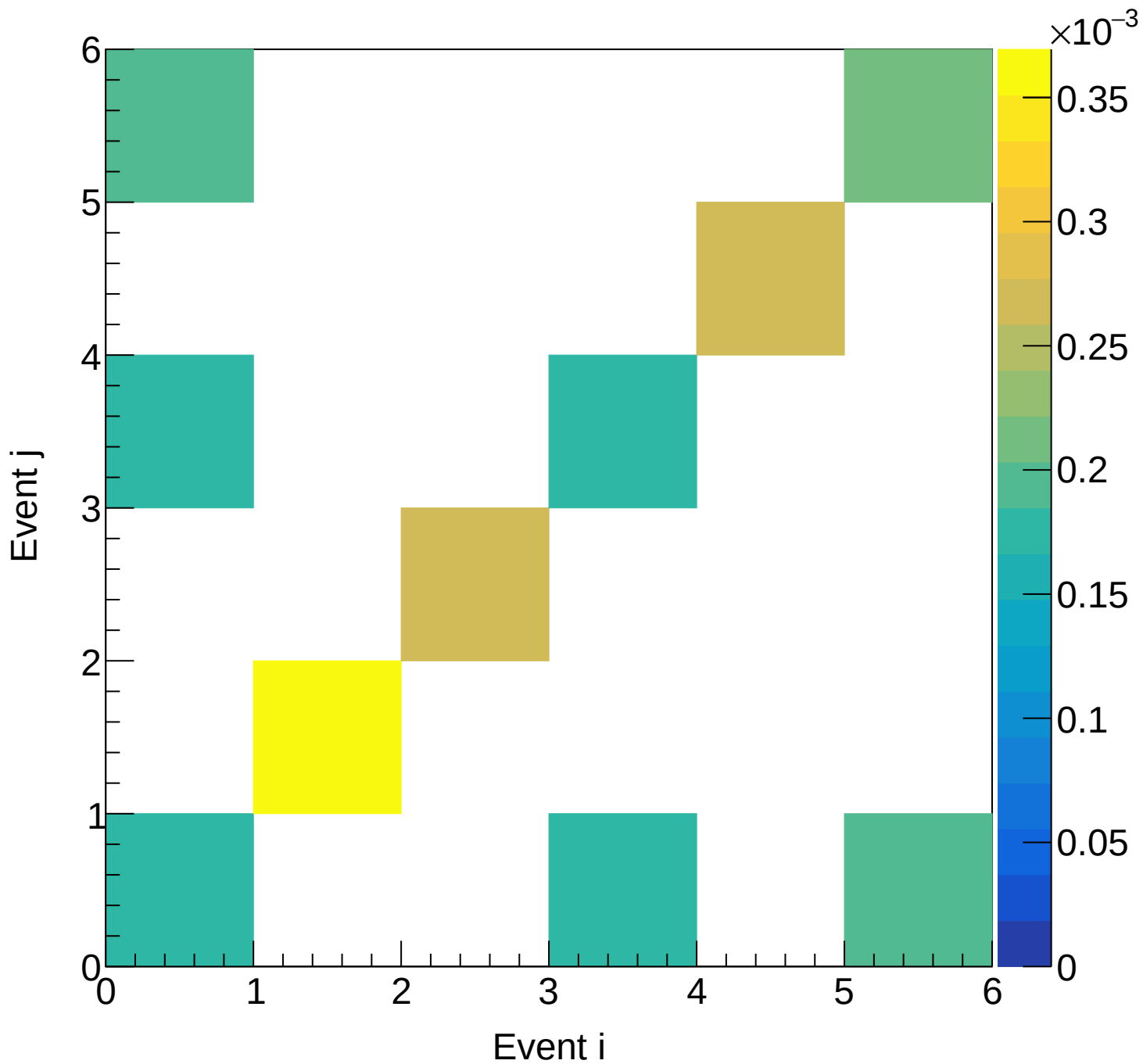
LD2 (mix) Covariance | M: [5.4, 5.7) xF: [-0.05, 0.00)
