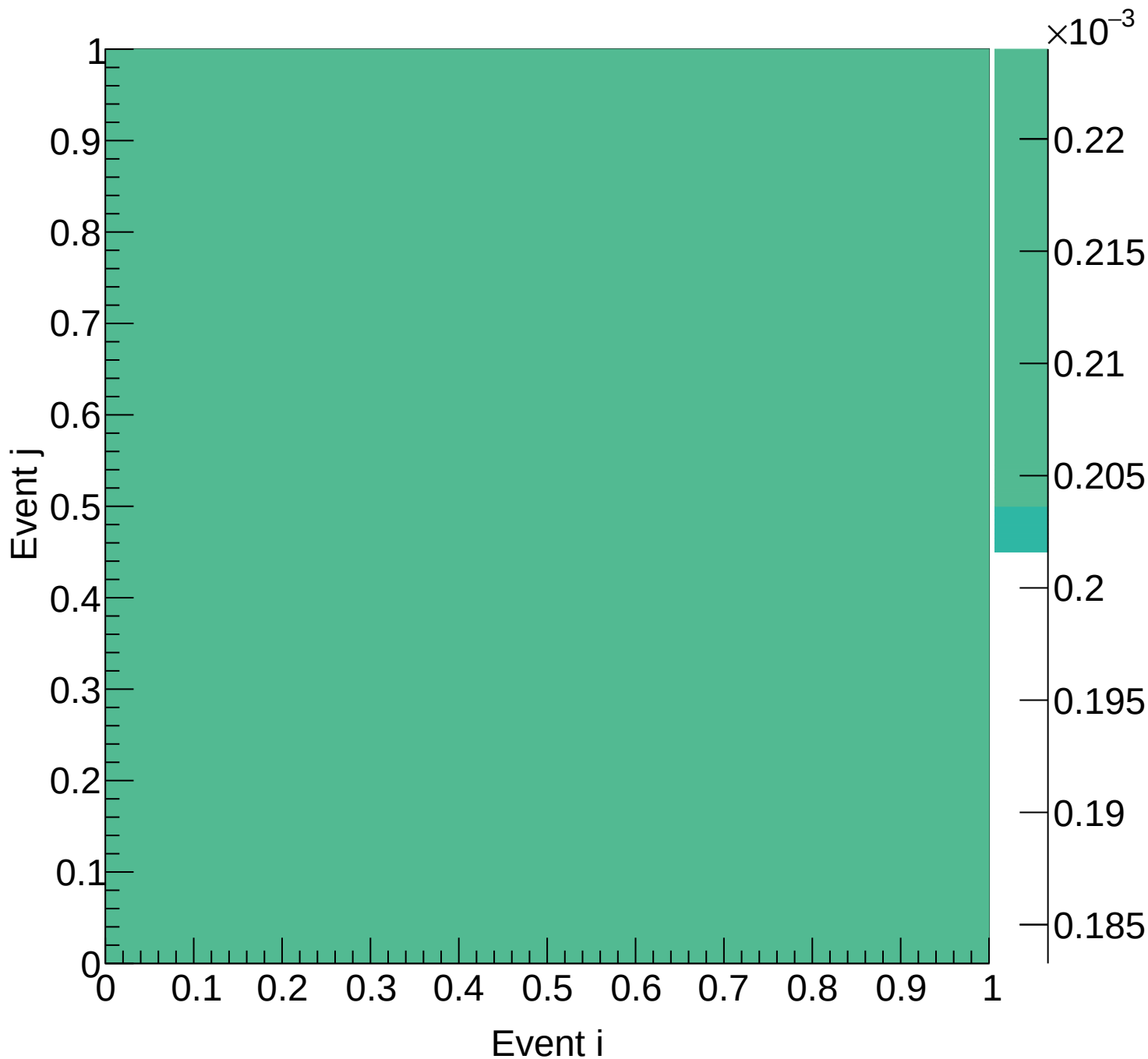
LD2 (mix) Covariance | M: [6.3, 6.6] xF: [-0.05, 0.00)
