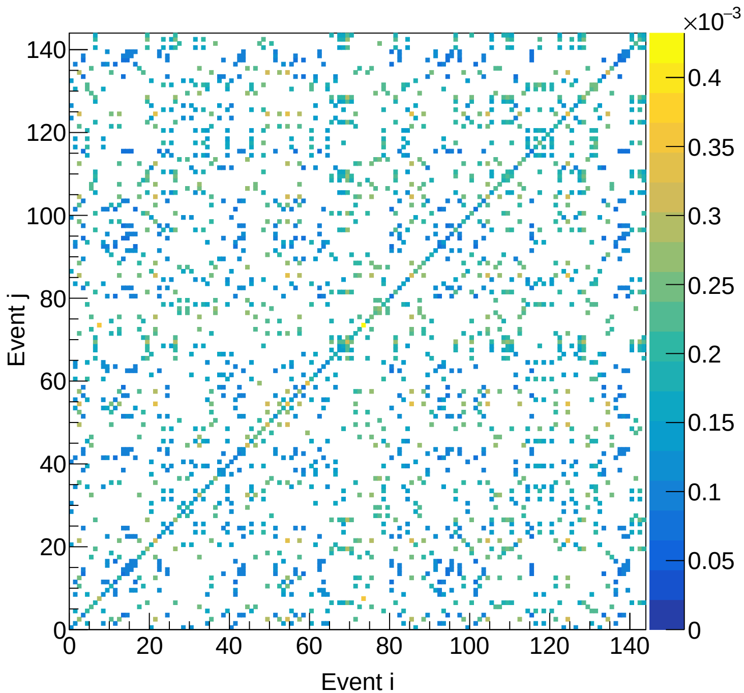
LD2 (mix) Covariance | M: [3.9, 4.2) xF: [0.45, 0.50)
