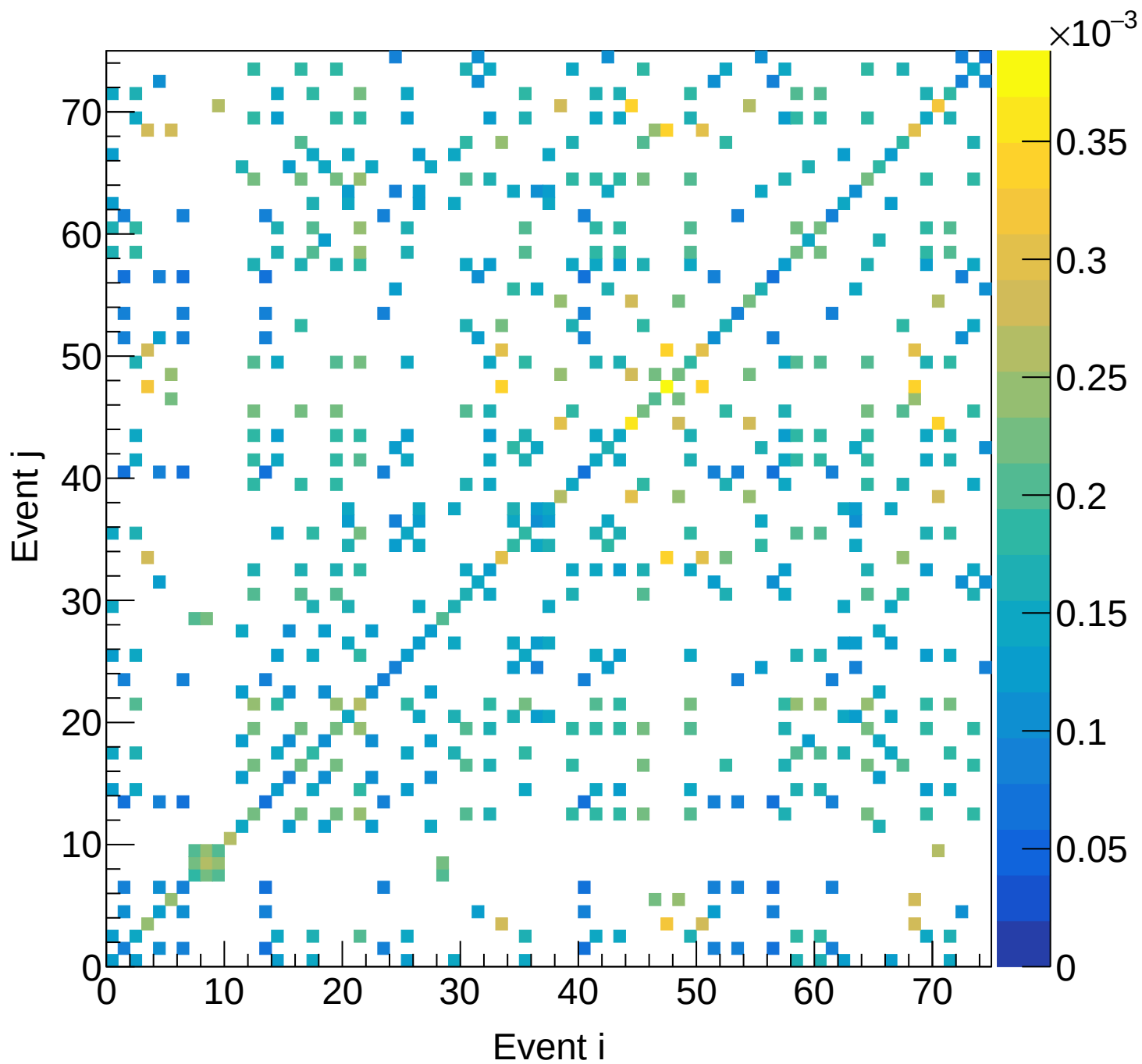
LD2 (mix) Covariance | M: [4.2, 4.5) xF: [0.45, 0.50)
