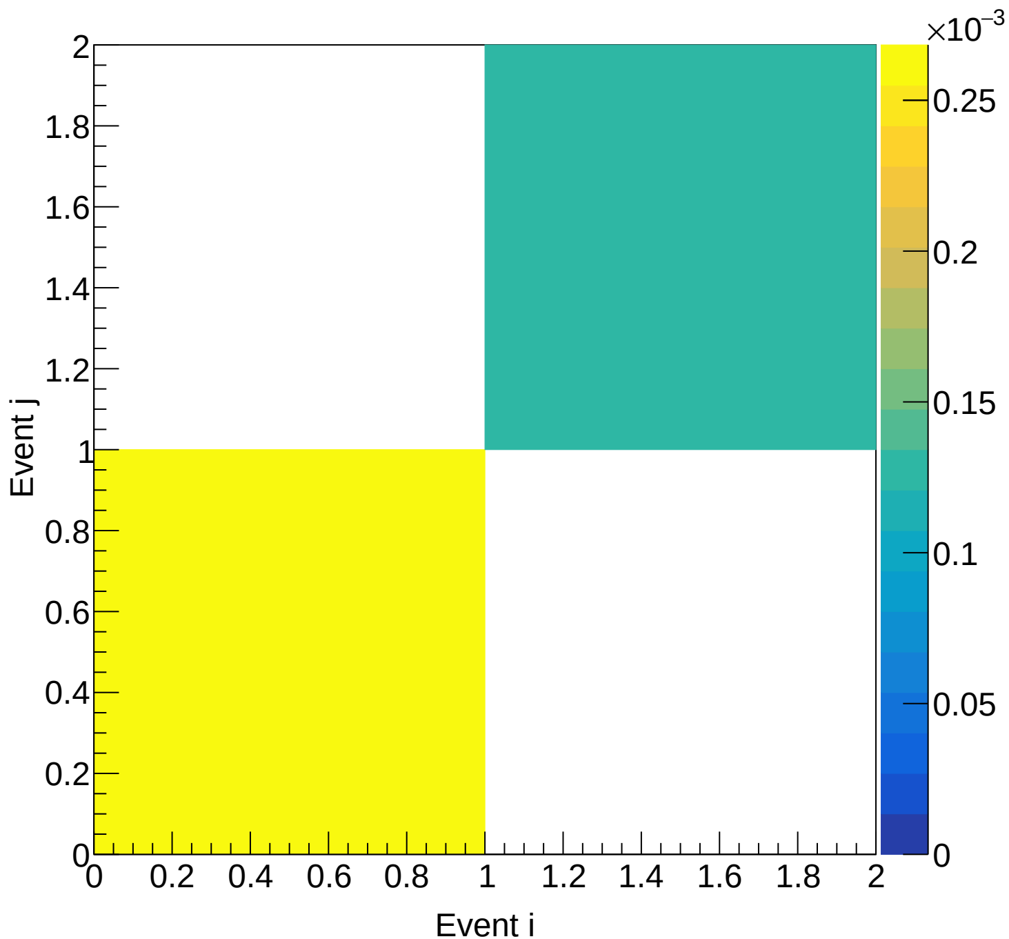
LD2 (mix) Covariance | M: [6.9, 7.5] xF: [0.50, 0.55)
