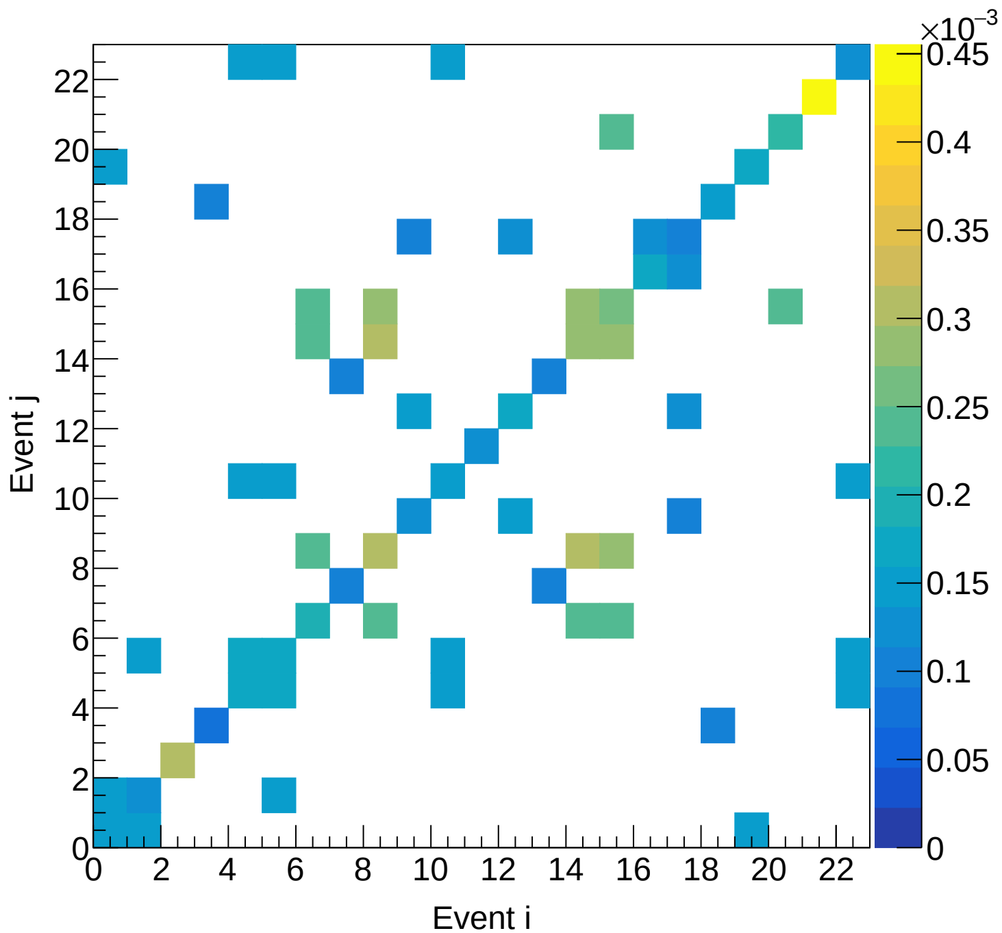
LD2 (mix) Covariance | M: [4.5, 4.8) xF: [0.50, 0.55)
