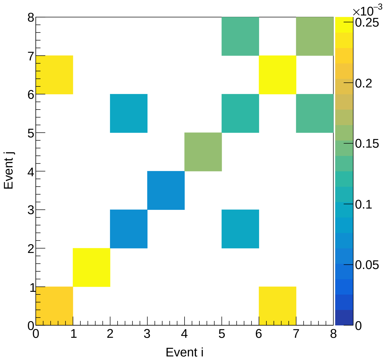
LD2 (mix) Covariance | M: [5.1, 5.4) xF: [0.50, 0.55)
