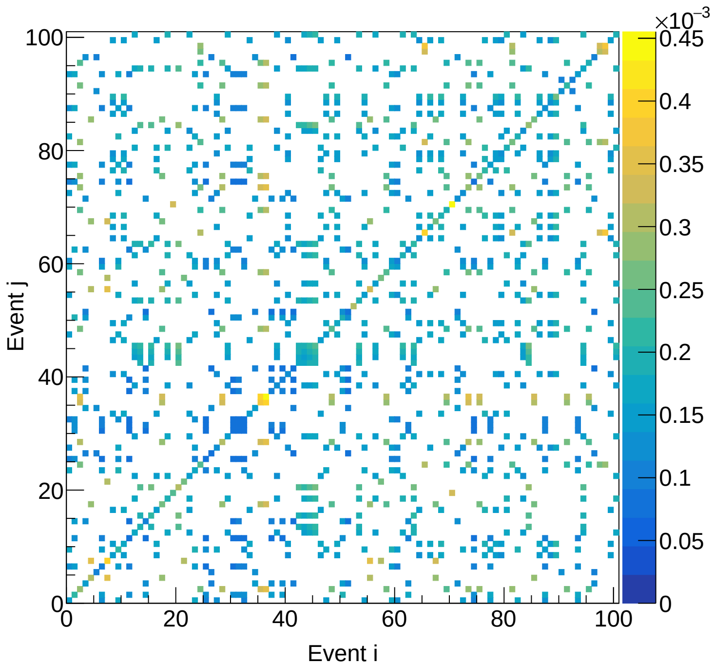
LD2 (mix) Covariance | M: [3.9, 4.2] xF: [0.55, 0.60)
