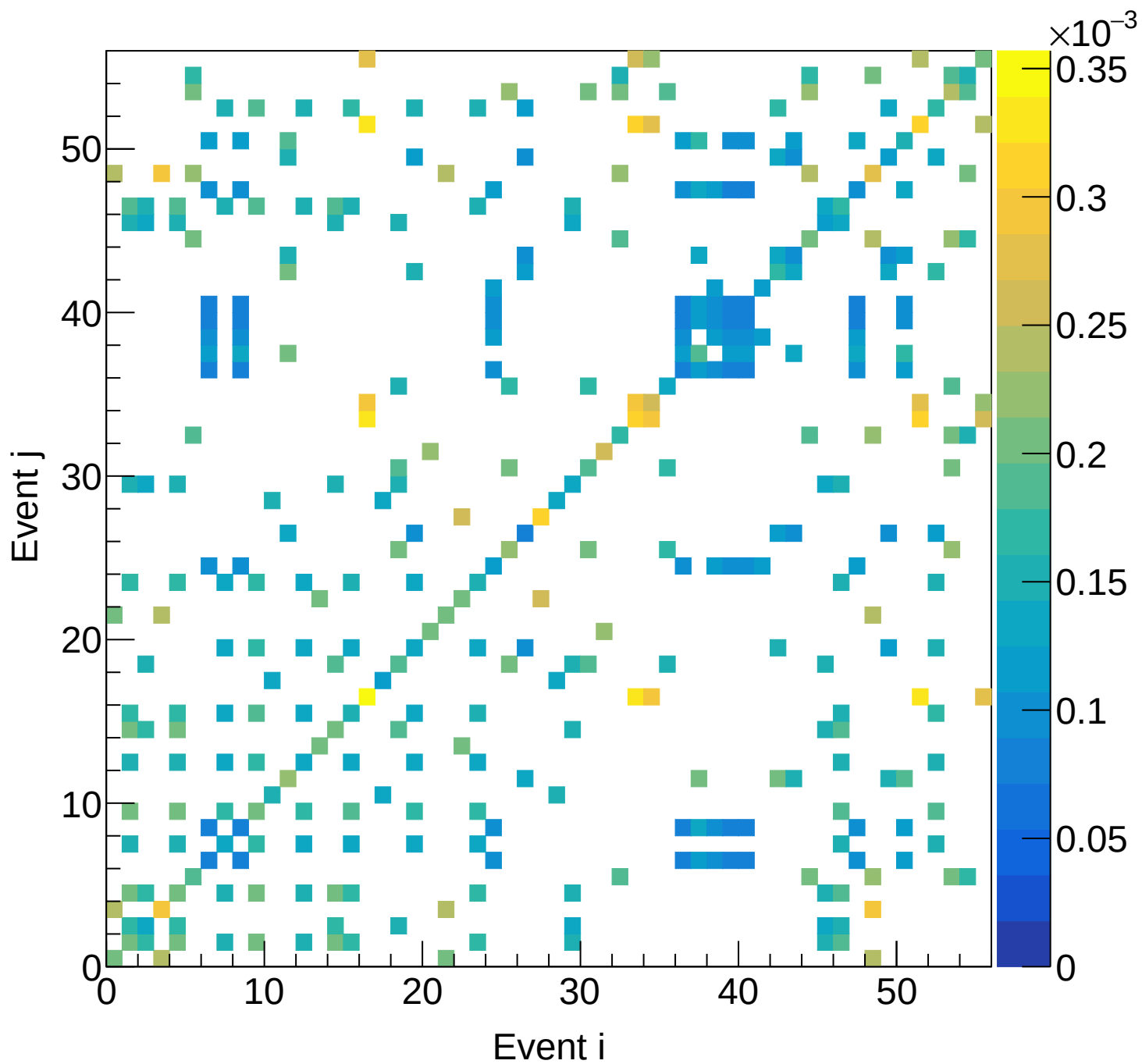
LD2 (mix) Covariance | M: [4.2, 4.5) xF: [0.55, 0.60)
