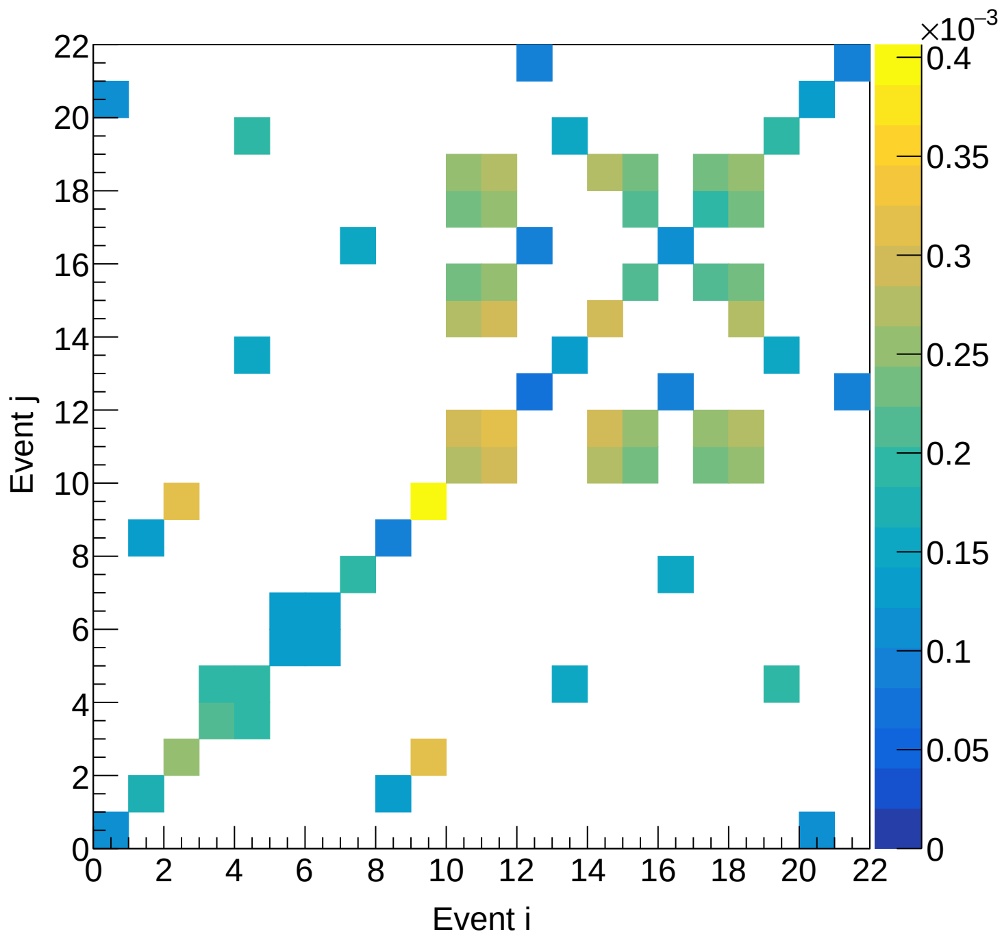
LD2 (mix) Covariance | M: [4.5, 4.8] xF: [0.55, 0.60)
