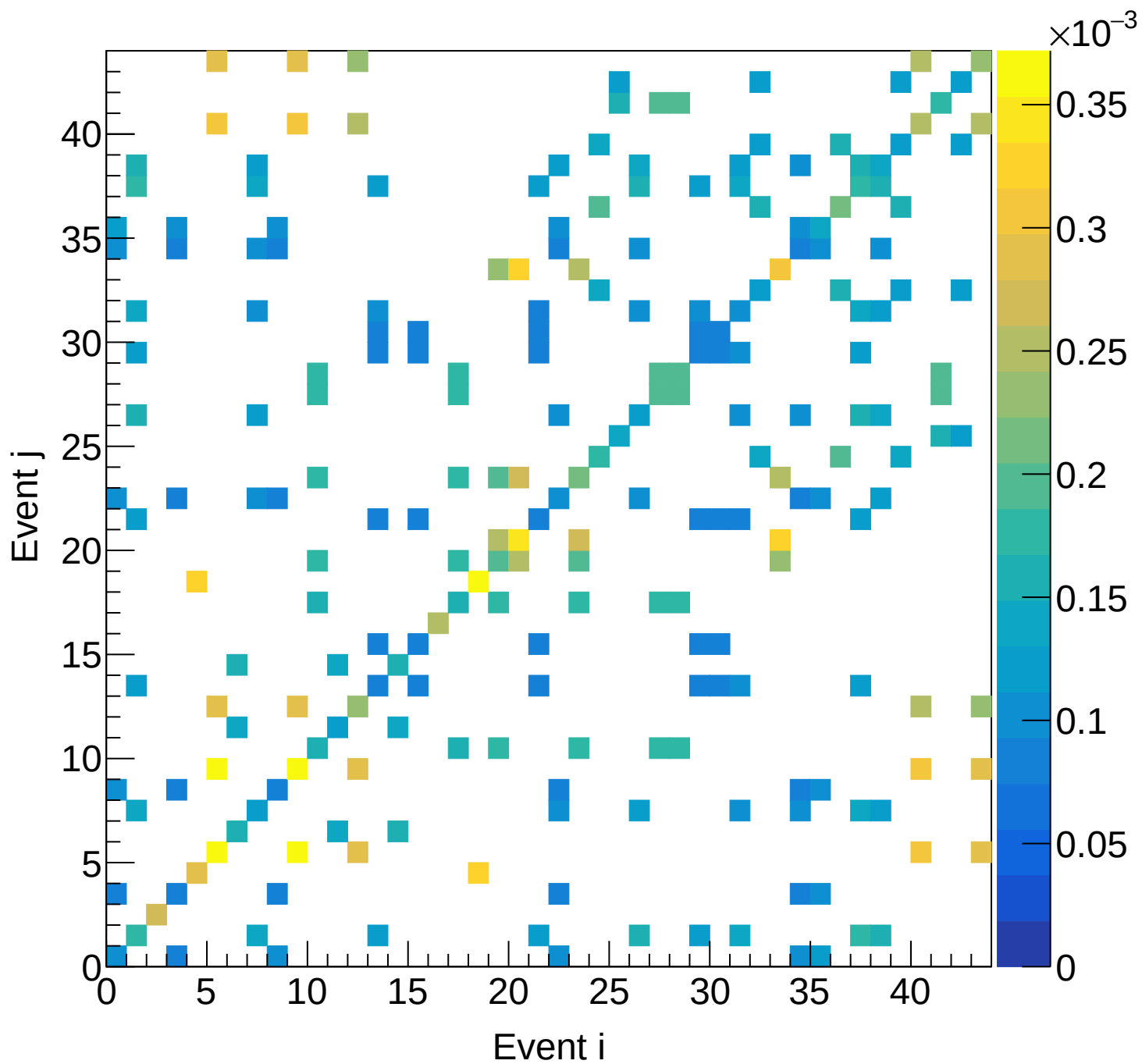
LD2 (mix) Covariance | M: [4.2, 4.5) xF: [0.60, 0.65)
