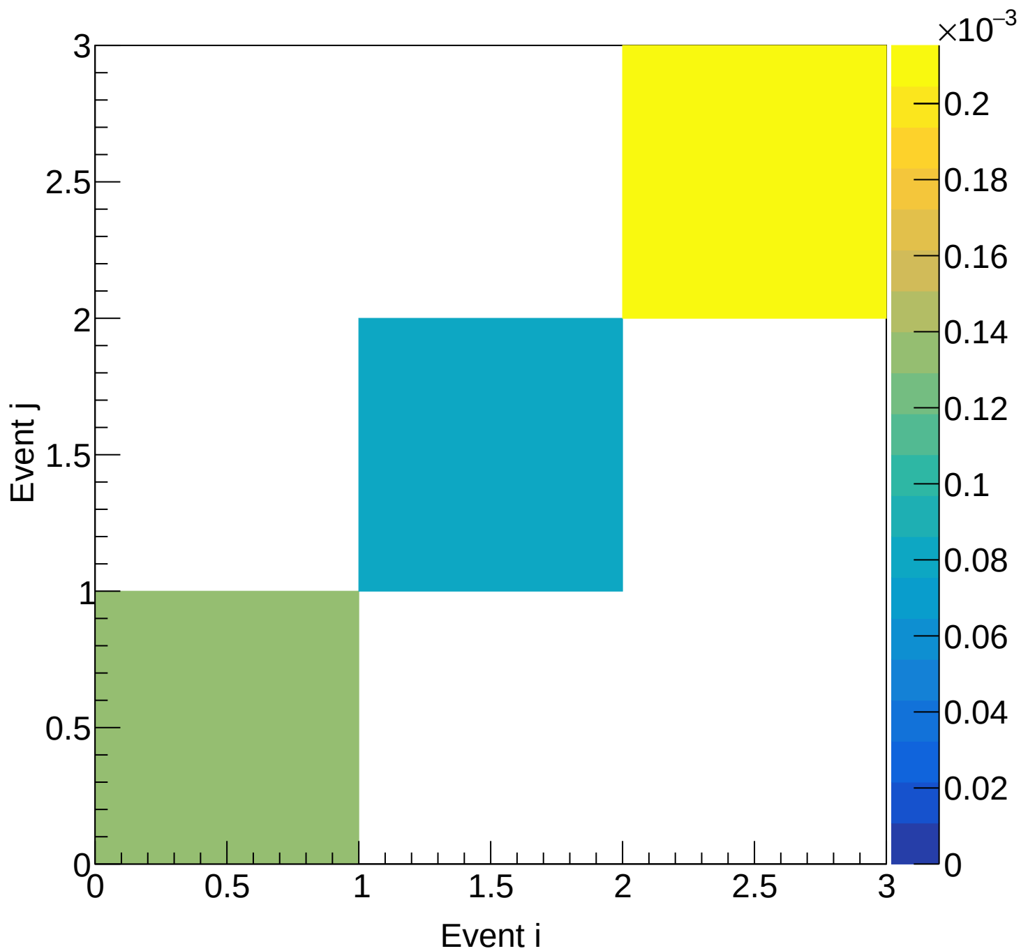
LD2 (mix) Covariance | M: [5.4, 5.7) xF: [0.60, 0.65)
