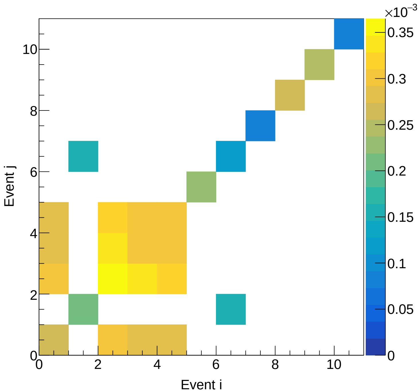
LD2 (mix) Covariance | M: [4.5, 4.8] xF: [0.65, 0.70)
