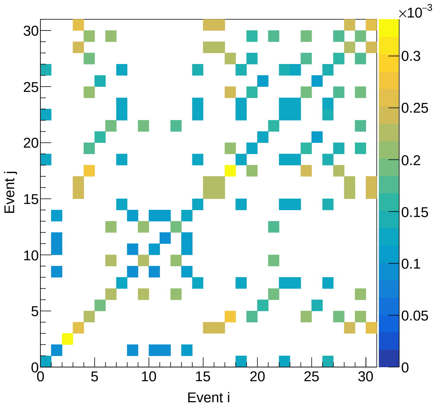
LD2 (mix) Covariance | M: [3.9, 4.2) xF: [0.70, 0.75)
