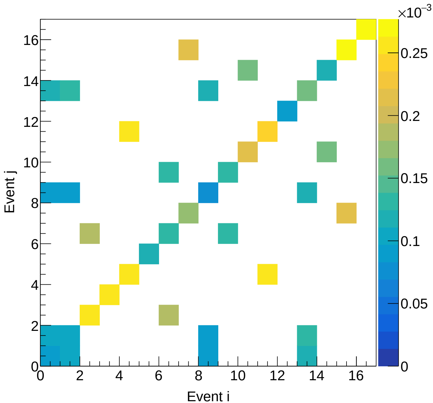
LD2 (mix) Covariance | M: [4.2, 4.5] xF: [0.70, 0.75)
