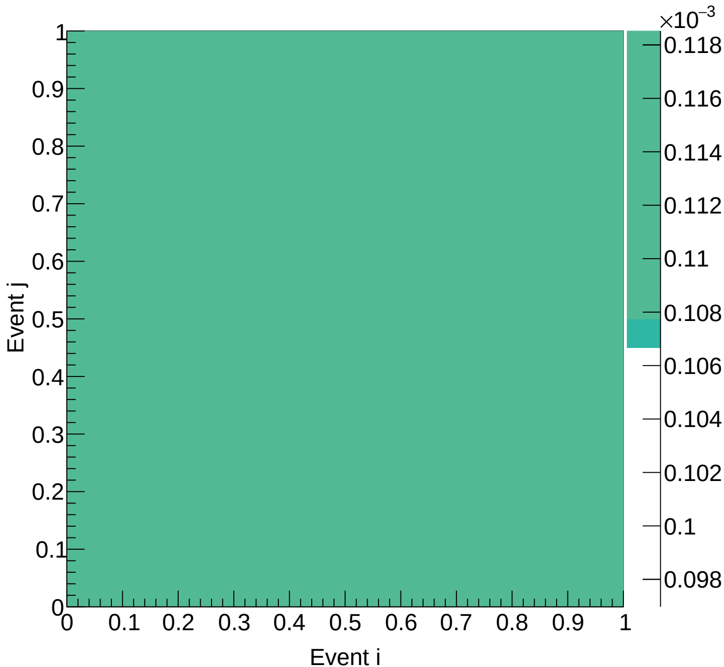
LD2 (mix) Covariance | M: [6.9, 7.5] xF: [0.70, 0.75)
