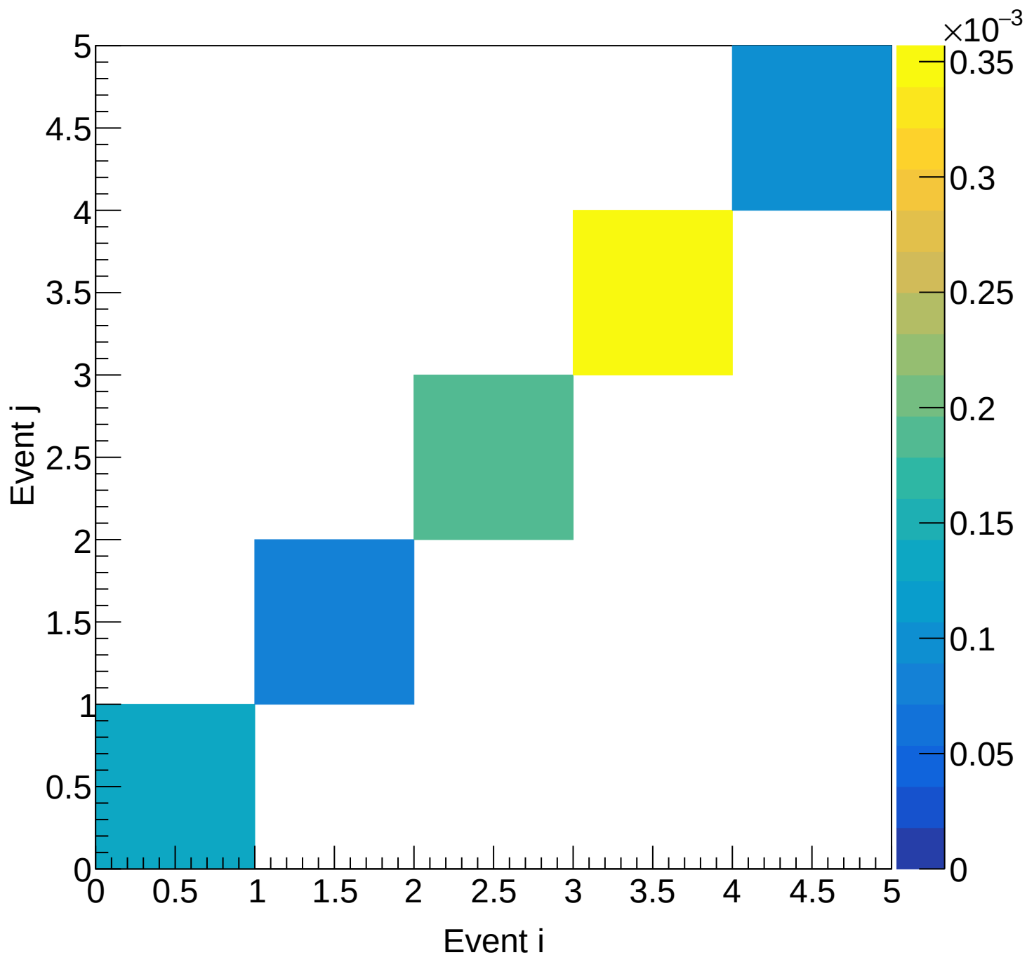
LD2 (mix) Covariance | M: [4.8, 5.1) xF: [0.70, 0.75)
