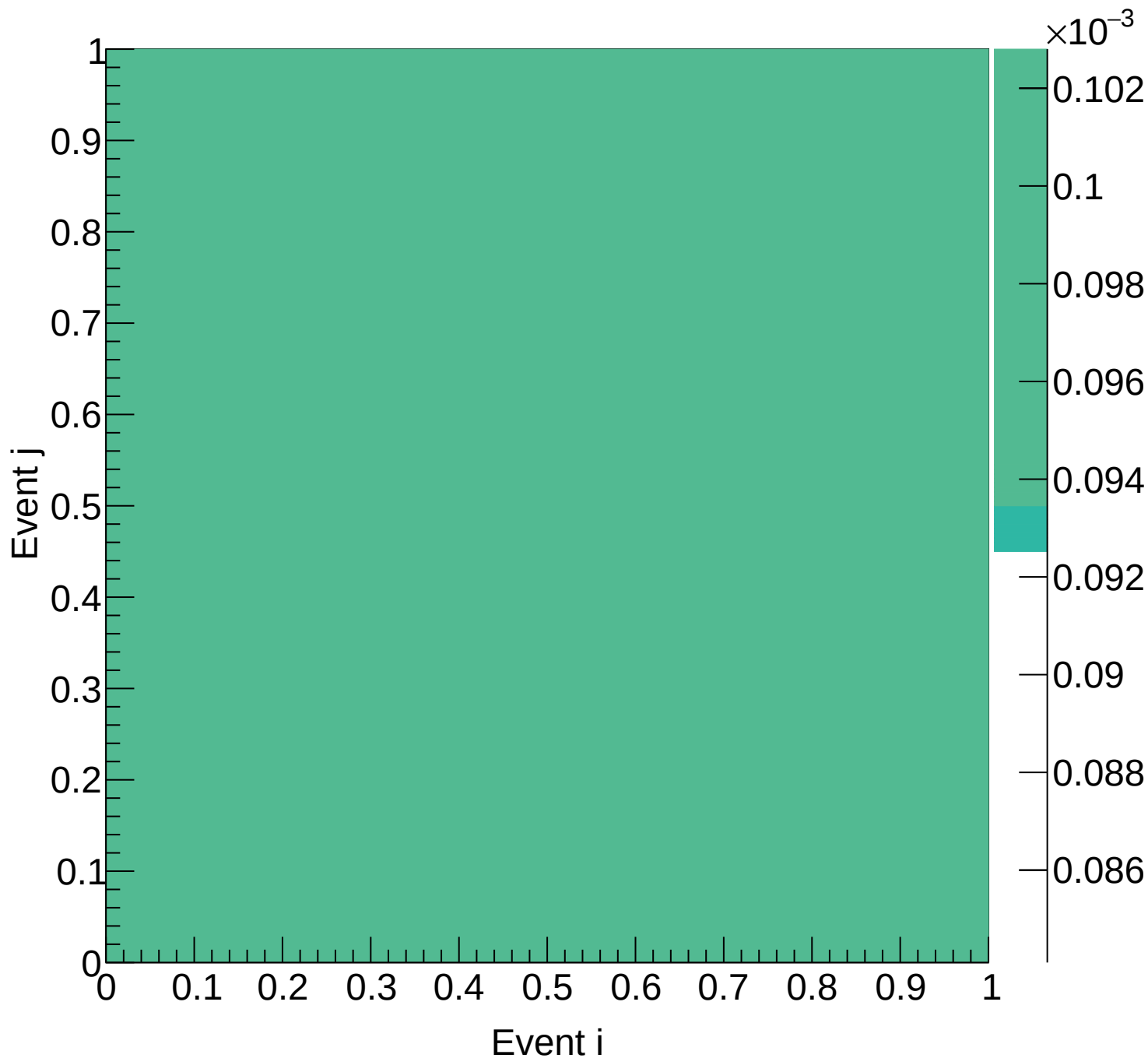
LD2 (mix) Covariance | M: [5.1, 5.4) xF: [0.70, 0.75)
